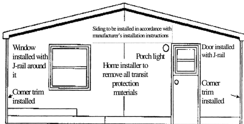
Figure A to Subchapter I, Section I – Exterior Close-up Installation of Field-Applied Horizontal Lap Siding
