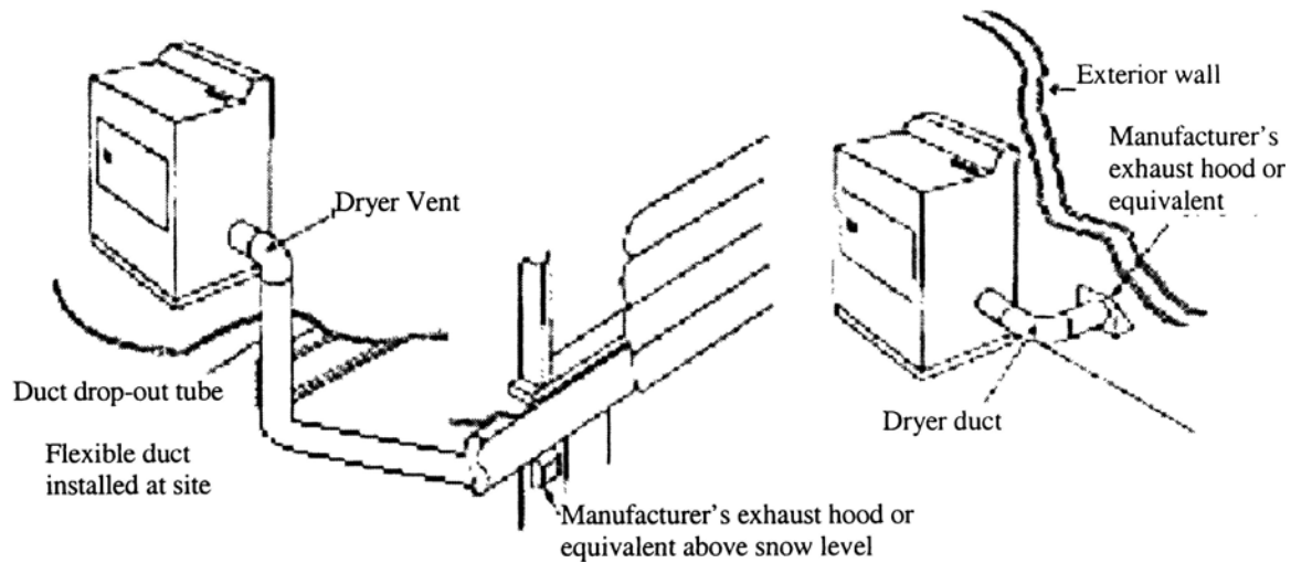
Figure to Subchapter F, Section III – Optional Appliances: Dryer Exhaust System
