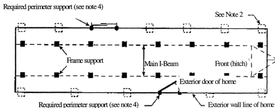
Figure A to Subchapter D, Section XII – Footings Typical Blocking Diagram for Single Section Homes
