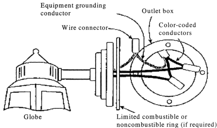
Figure B to Subchapter H, Section II – Miscellaneous Lights and Fixtures Typical Installation of Surface-Mounted Exterior Lighting Fixture
