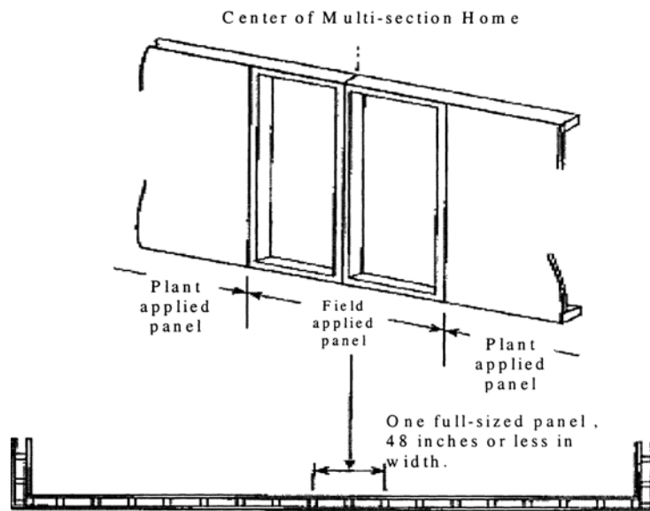
Figure to Subchapter I, Section III – Interior Close-up Installation of Interior Field-Applied Panels
