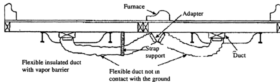
Figure A to Subchapter G, Section VI – Ductwork Connections Crossover Duct Installation With Two Connecting Ducts
