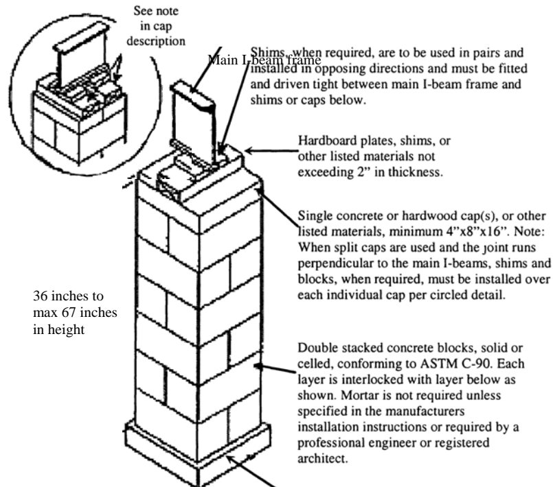
Figure B to Subchapter D, Section VI – Design Procedures for Concrete Block Piers: Typical Footing and Pier Installation, Double Concrete Block
