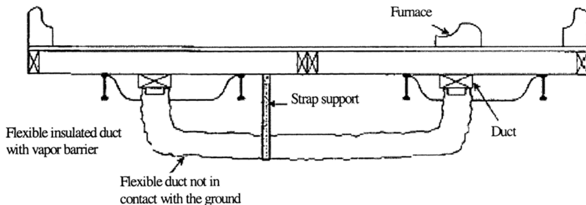
Figure B to Subchapter G, Section VI – Ductwork Connections Crossover Duct Installation with One Connecting Duct
