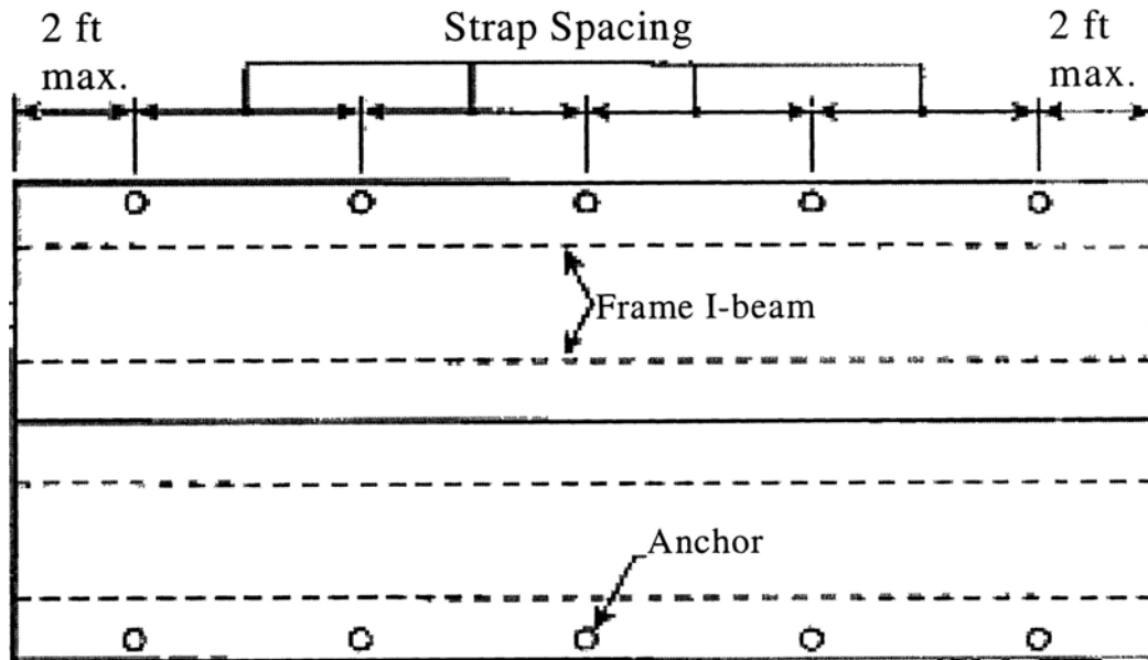
Figure A to Subchapter E, Section II – Ground Anchor Installations Ground Anchor Locations and Spacing (Plan View)
