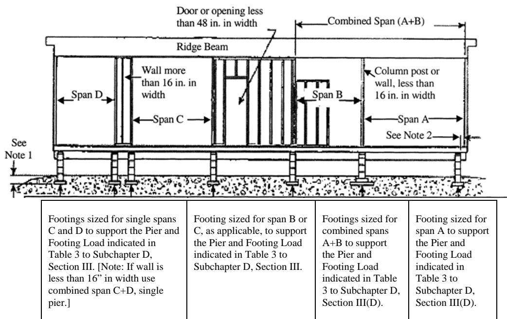
Figure A to Subchapter D, Section X – Pier Location and Spacing: Typical Mate-Line Column Pier and Mating Wall Support When Frame Only Blocking is Required
