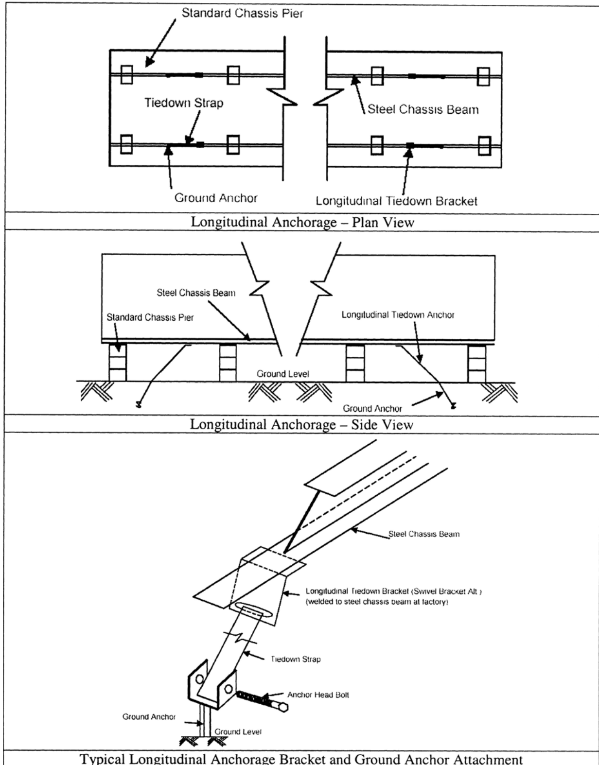
Figure C to Subchapter E, Section II – Ground Anchor Installation Longitudinal Anchoring
