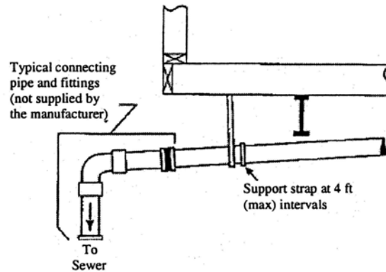
Figure to Subchapter J, Section II – Connection to Site Sewer
