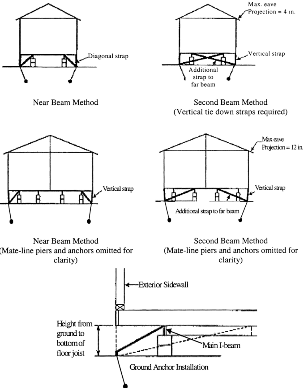
Figure B to Subchapter E, Section II – Ground Anchor Installation Anchor Strap and Pier Relationship
