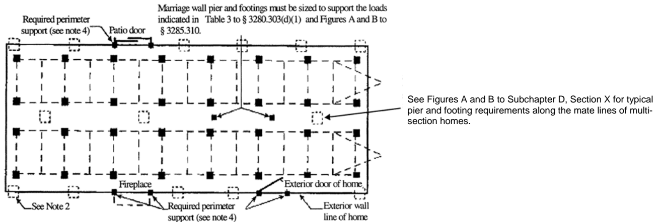
Figure B to Subchapter D, Section XII – Footings Typical Blocking Diagram for Multi-section Homes
