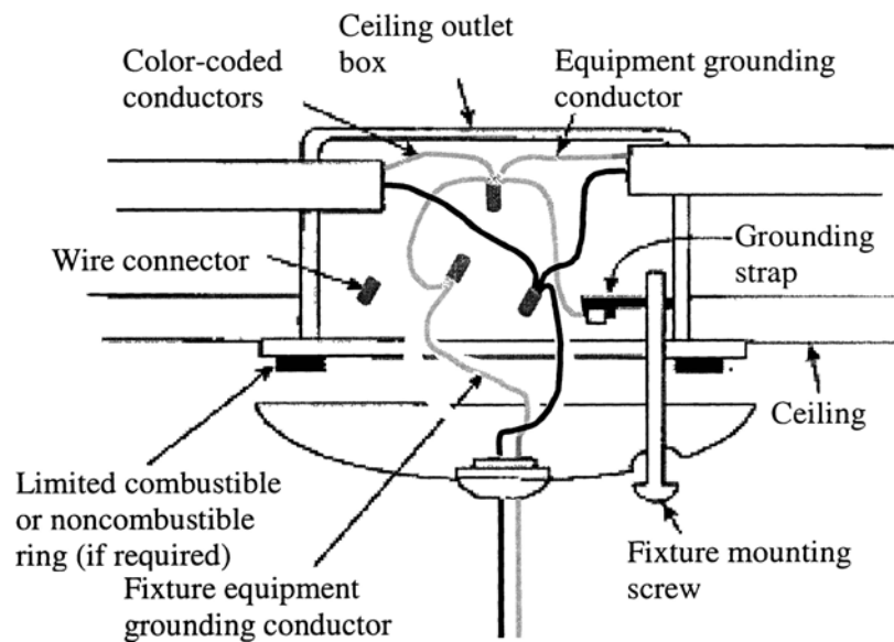
Figure A to Subchapter H, Section II – Miscellaneous Lights and Fixtures Typical Installation of Chain-Hung Lighting Fixture
