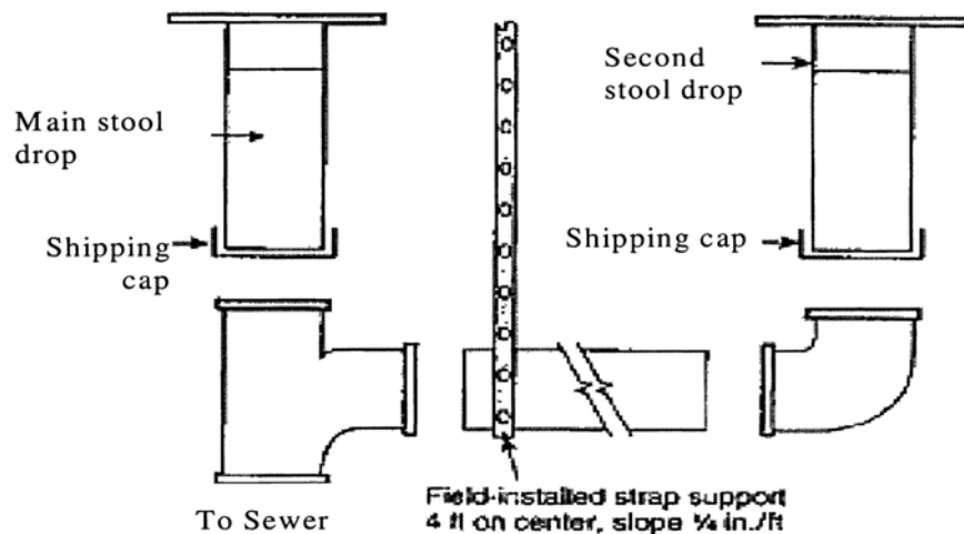
Figure to Subchapter G, Section IV – Drainage Systems Drain Pipe Slope and Connections
