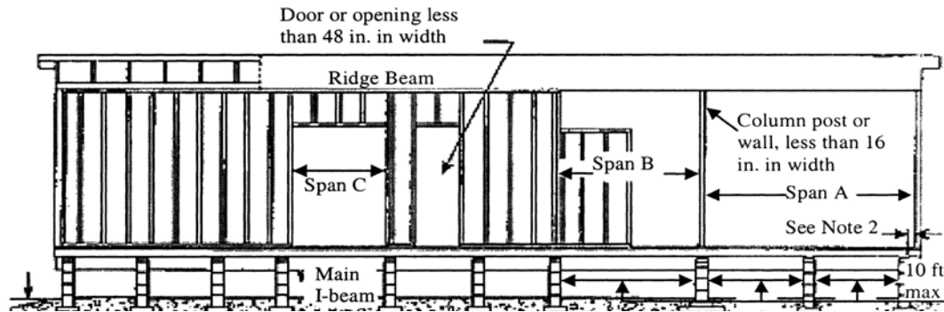
Figure B to Subchapter D, Section X – Pier Location & Spacing: Typical Mate-Line Column Pier and Mating Wall Support When Perimeter Blocking is Required
