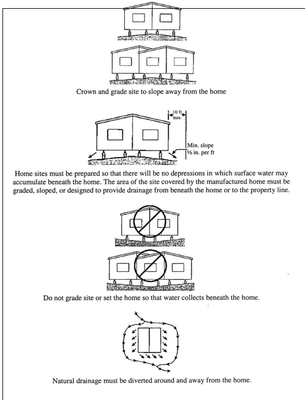
Figure to Subchapter C, Section III – Site Drainage
