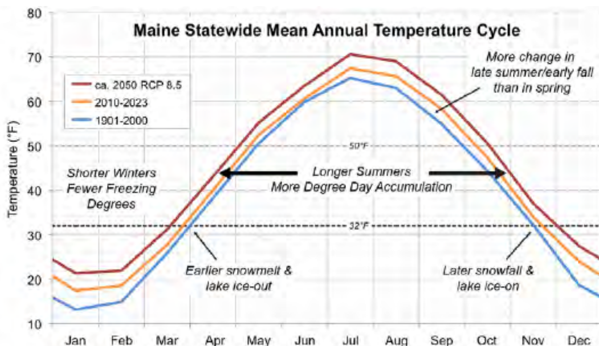
Figure 11.5: Maine Statewide Mean Annual Temperature Cycle
