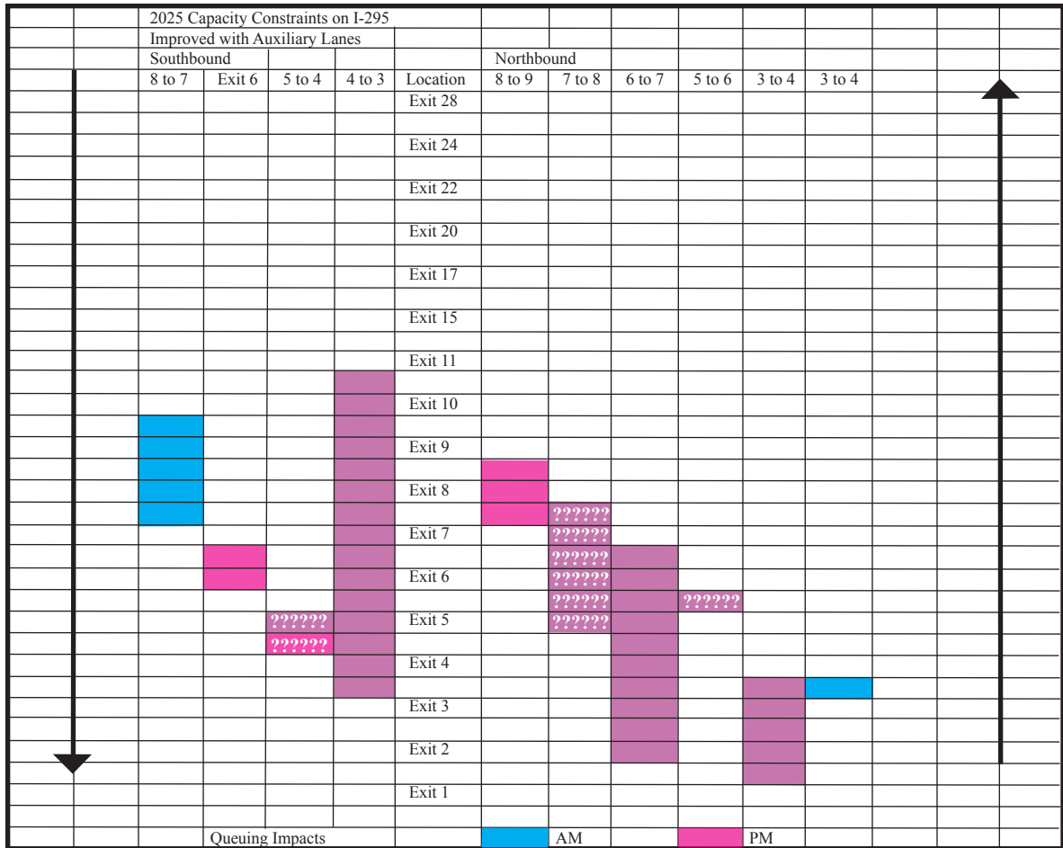
Figure 4.1: 2025 Auxiliary Lanes - Capacity Constraints Queuing Reductions
