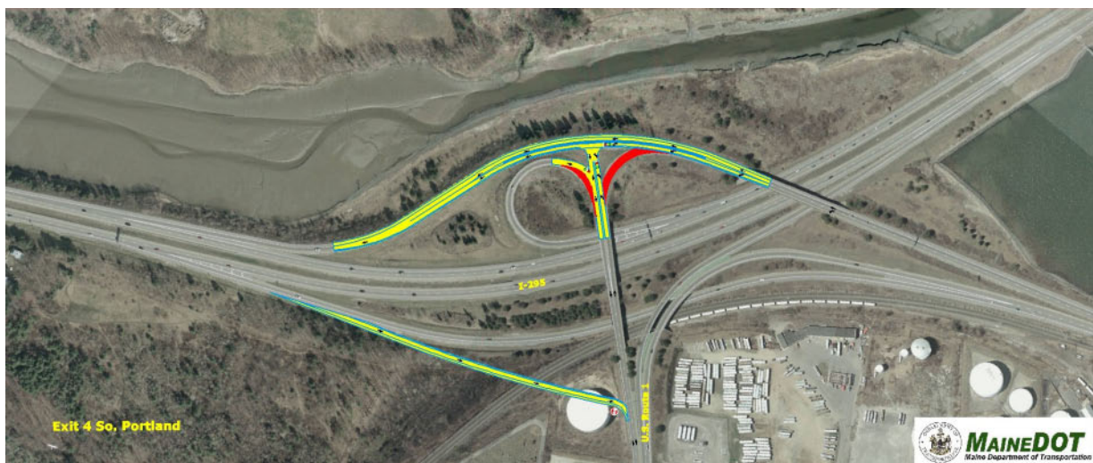
Figure 4.8 Exit 4 Improvement Concept (enlarged in Appendix 23)
