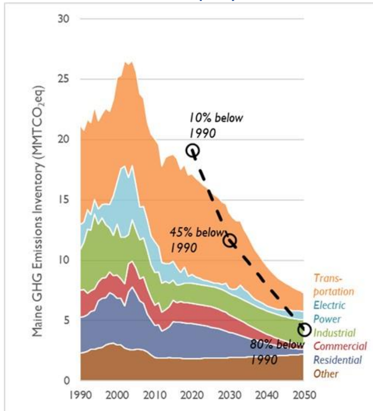
Figure 5. Economy-wide greenhouse gas emissions for the decarbonization policy scenario.
