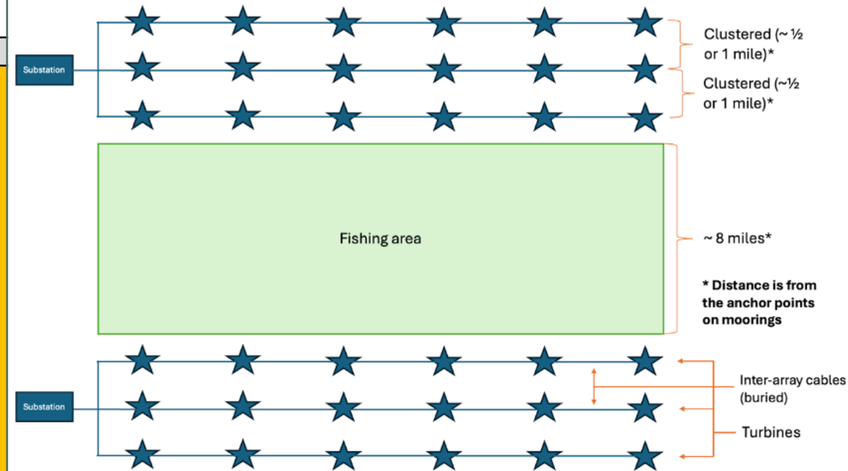
Draft layout
