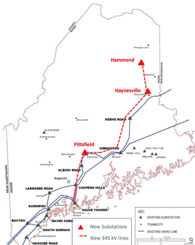
Figure 18. Northern Maine Renewable Integration Concept 50
