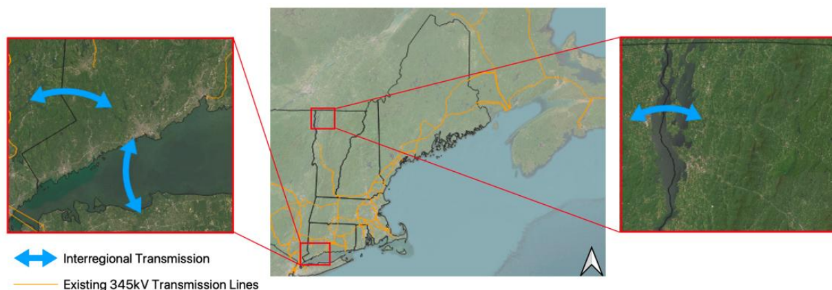
Figure 4: LTP Interregional Transmission as Potential Solutions to HLCs
