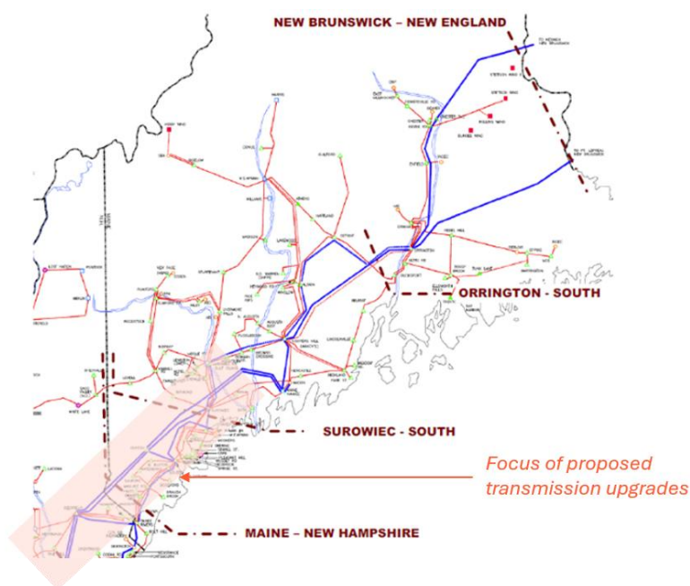
Figure 17. Maine Transmission Interfaces and Proposed LTTP Upgrade Areas 49
