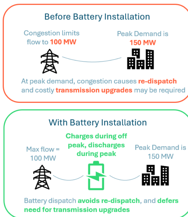
Figure 25. Storage as a Transmission Asset (SATA) Illustration
