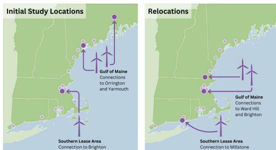
Figure 20. Offshore Wind Interconnection Locations Studied in ISO-NE's Offshore Wind Analysis 52
