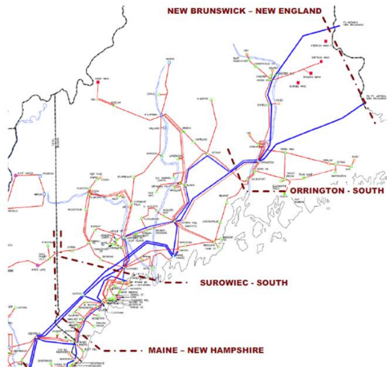
Figure 14. Key Transmission Interfaces within Maine and between Maine and the Rest of New England 48
