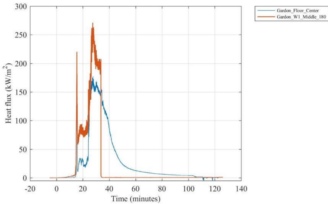
Figure F 14. Heat flux measured by Gardon gauges located inside the compartment.
