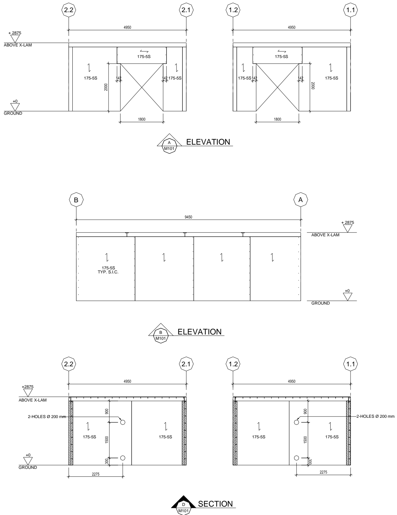
Figure 4. Elevation and Section View of CLT Compartments.
