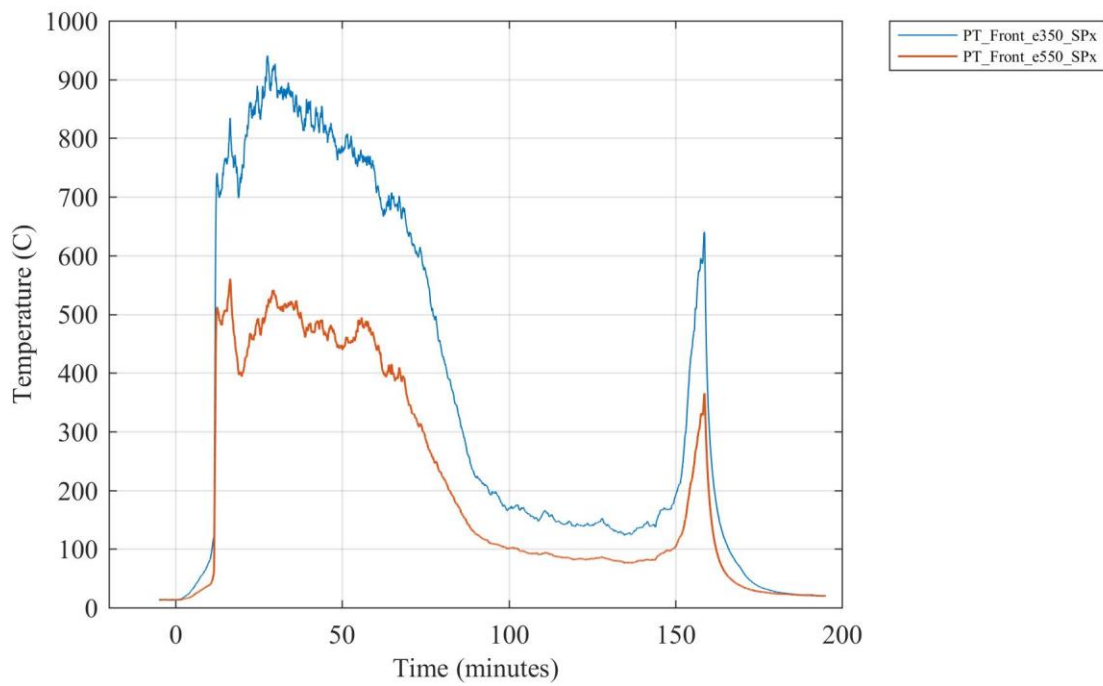
Figure H 30. Plate thermometer temperatures 350 cm and 550 cm above the floor above the doorway.
