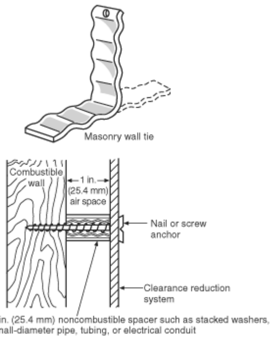
FIGURE 12.6.2.1(c) Masonry Clearance Reduction System.
