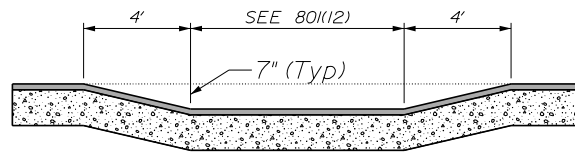
~ SECTION B-B ~ (not to scale)
