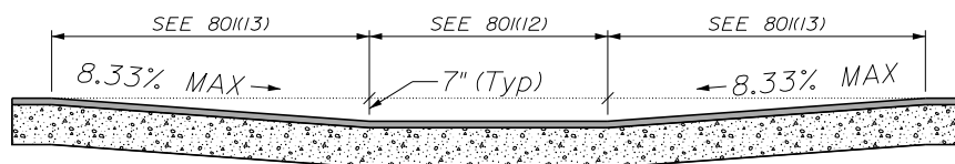
~ SECTION B-B ~ (not to scale)
