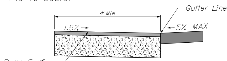
~ SECTION A-A ~ (not to scale)
