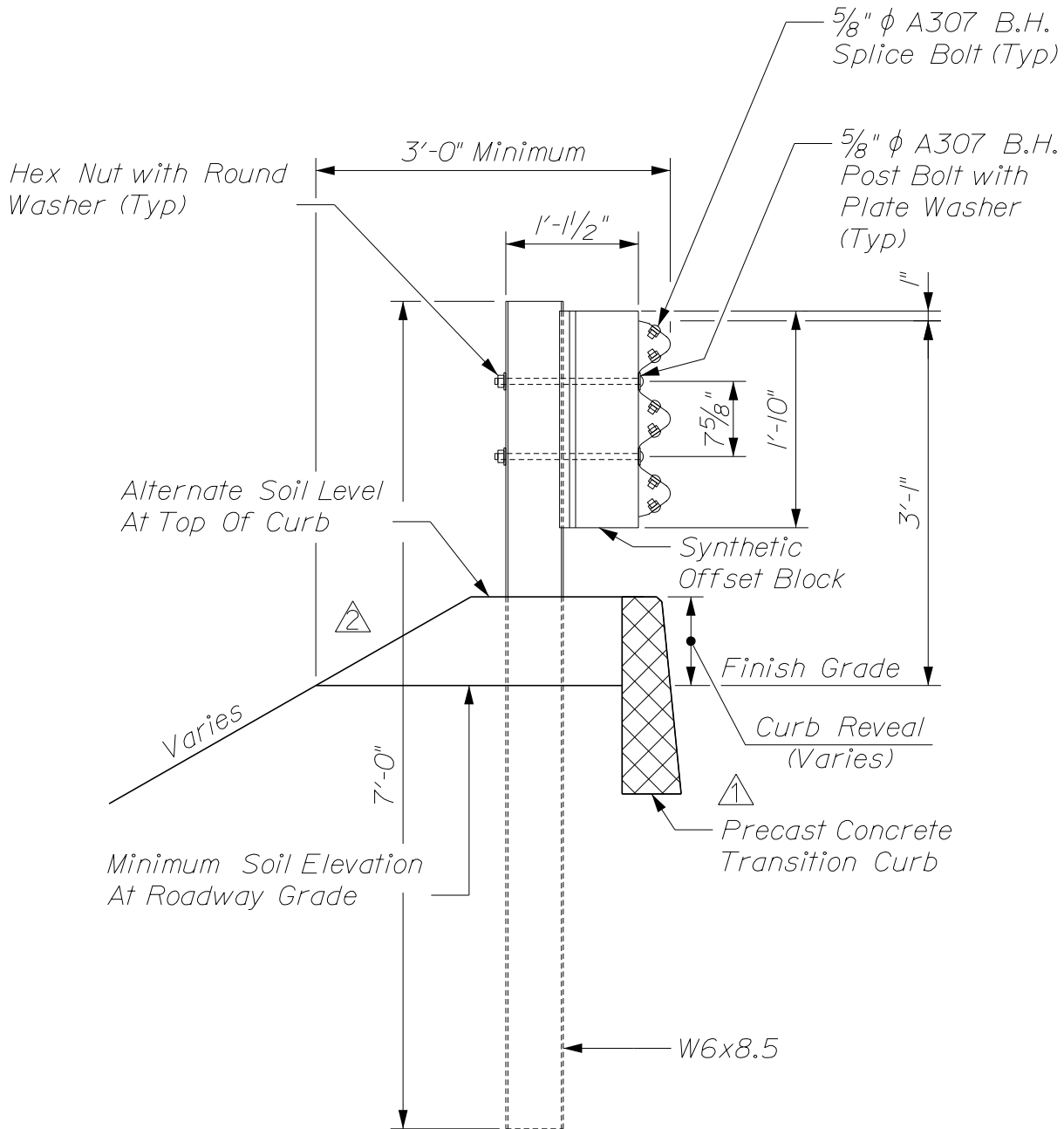
~ SECTION A-A ~ (POST RAIL ASSEMBLY)
