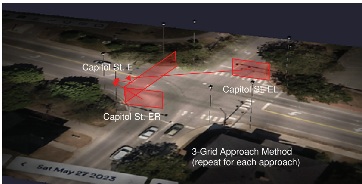
Figure 10-1. Illustration. Isometric Illustration of the 3-Grid Approach method for one leg of an intersection.
