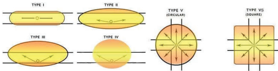
Figure 3-11. IES Classifications for a luminaire's transverse distribution of light. (IES RP-8-21)
