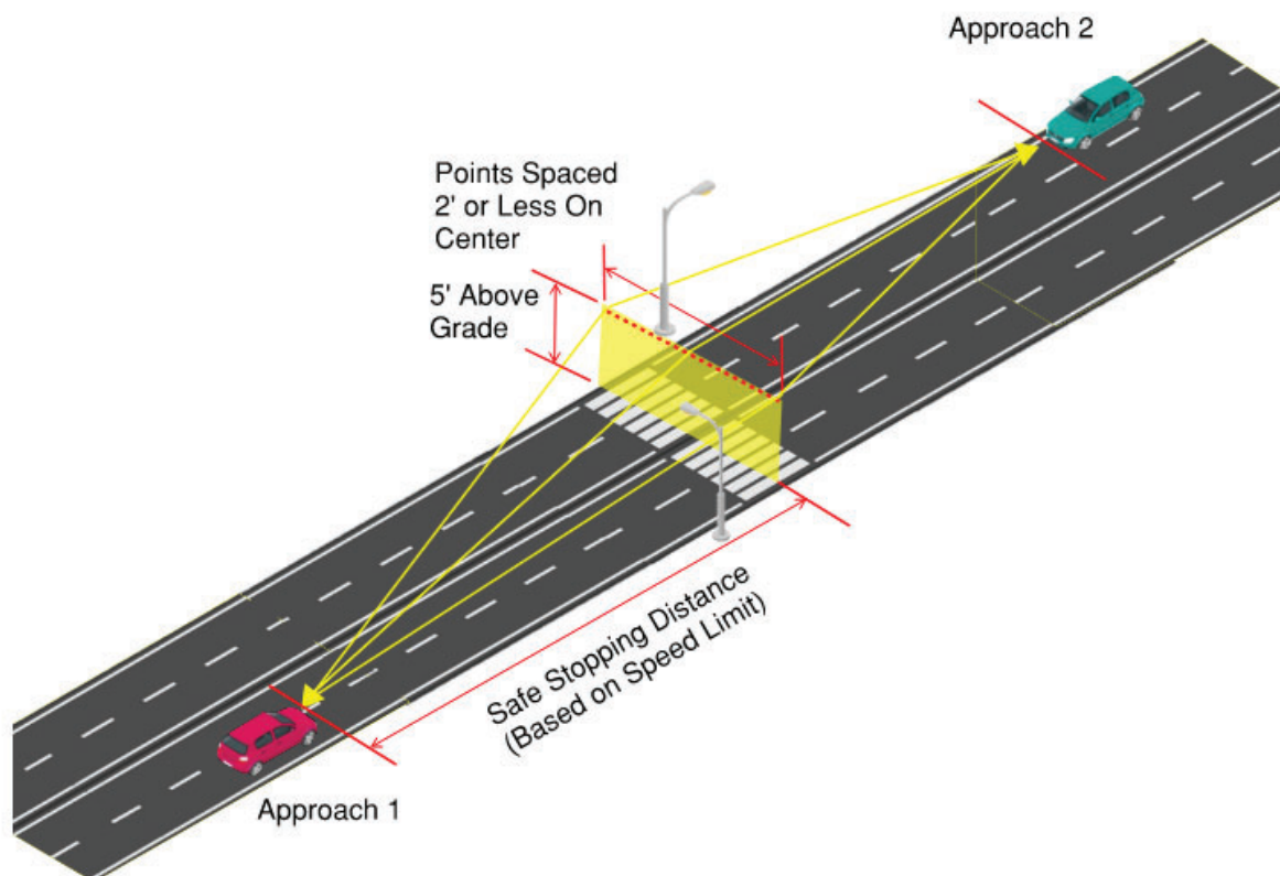
Figure 12-3. Illustration. One vertical illuminance calculation grid across the entire roadway for each approach.
