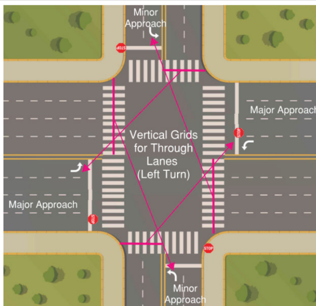
Figure 10-4. Illustration. Vertical Grids per Left Turn.
