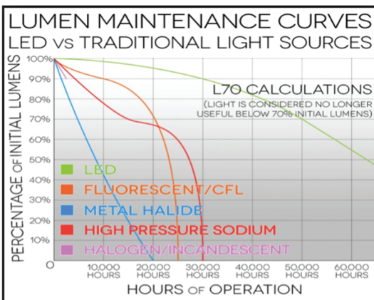
Figure 2-21. Graph. Example of lumen depreciation curves for various types of light sources (Source: foreverlight.com )
