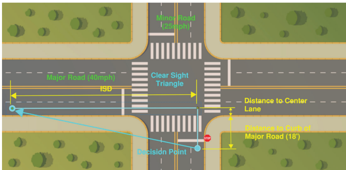
Figure 6-6. Illustration. Stop Control on Minor Road & Left Turn from Minor Road (AASHTO ISD Case B1, E, & F).
