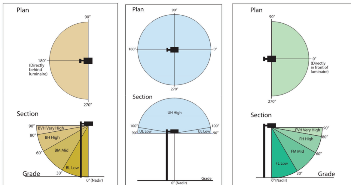
Figure 3-6. Illustration. Plan and elevation views of the distribution of backlight, uplight, and forward light and the range of degrees used to further classify each type. (IES RP-8-21, Ch.2, Fig. 2-27, 2-28, and 2-26)
