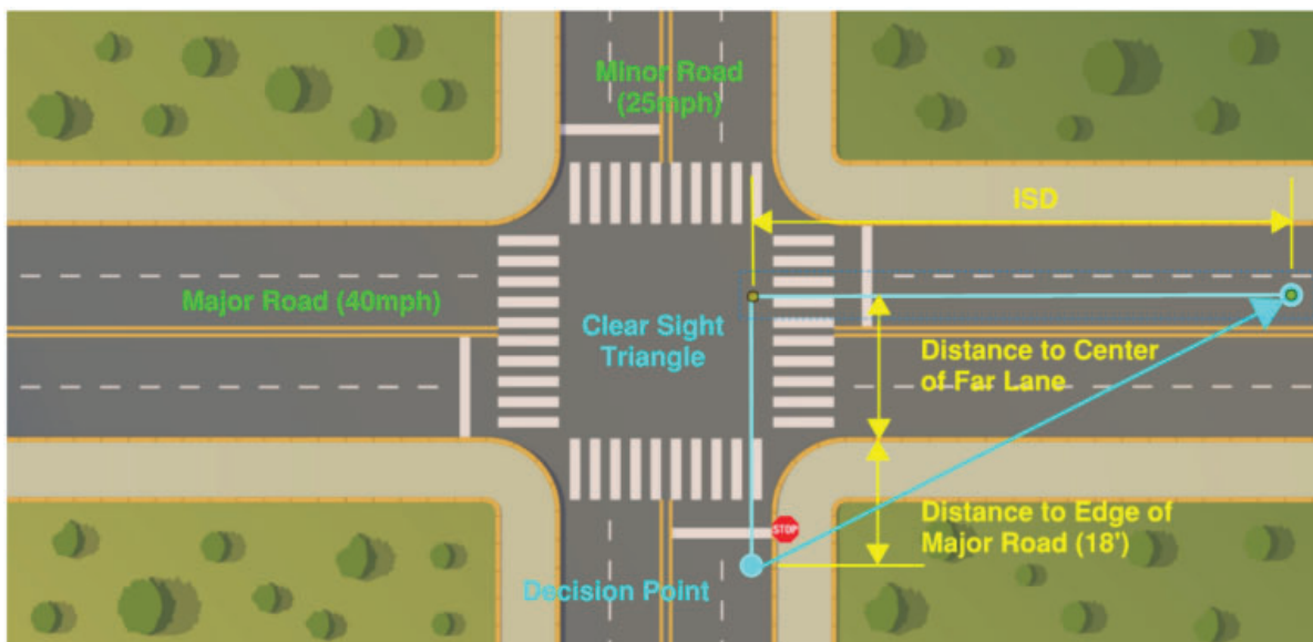
Figure 6-4. Illustration. Stop Control on Minor Road & Right Turn from Minor Road (AASHTO ISD Case B2, B3, E & F).
