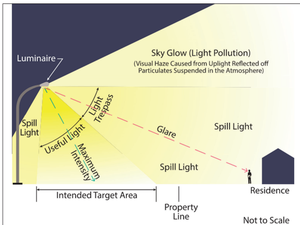
Figure 3-1. Illustration. The components of obtrusive light (not to scale). (Source: IES RP-8-21, Fig. 4-1.)
