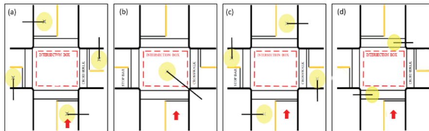
Figure 9-2. Illustration. Intersection lighting design evaluated in the FHWA-ICT-21-023 study. The intersection was illuminated with four lighting design configurations: (a) illuminated approach, (b) illuminated box, (c) illuminated exit, and (d) illuminated with luminaires on the signal mast arm. (FHWA-ICT-21-023, 2021)
