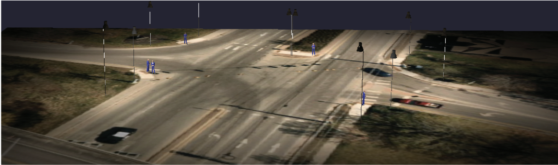
Figure 10-7. Rendering. The intersection of Main Street and Veterans Memorial Bridge in Lewiston, Maine. Due to the unique geometry of this intersection, there are 7 vertical illuminance grids required. The location and quantity of vertical calculation grids shall be based on the needs of each individual intersection and the flow of traffic.
