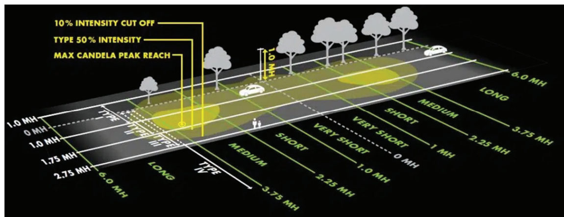
Figure 3-12. Illustration. IES Classifications for horizontal and vertical distributions of light in relation to its mounting height (Source: https://www.zgsm-china.com/blog/light-distribution-of-outdoor-luminaire-and-their-applications.html )
