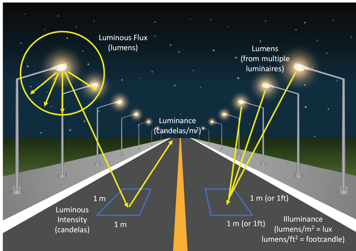
Figure 2-1. Illustration. Luminous flux, luminous intensity, illuminance, and luminance.
