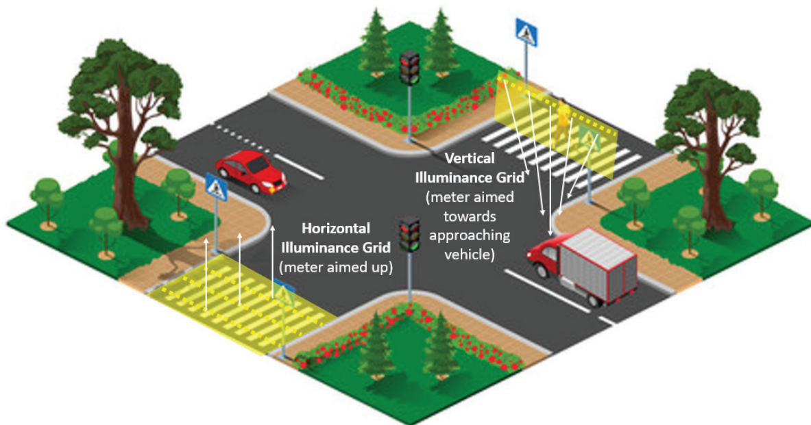
Figure 2-11. Illustration. Virtual meter aiming for horizontal and vertical calculation grids.
