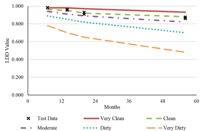
Figure 2-22. Graph. Measured dirt depreciation values compared with IES values compared with IES estimated values from RP-36-15, for five different environmental conditions. (Source: Robert G. Davis, Andrea M. Wilkerson, Bruce R. Kinzey 2019. Luminaire Dirt Depreciation (LDD): Field Data from Several Exterior Lighting Projects . LEUKOS, 15:1, 55-63)
