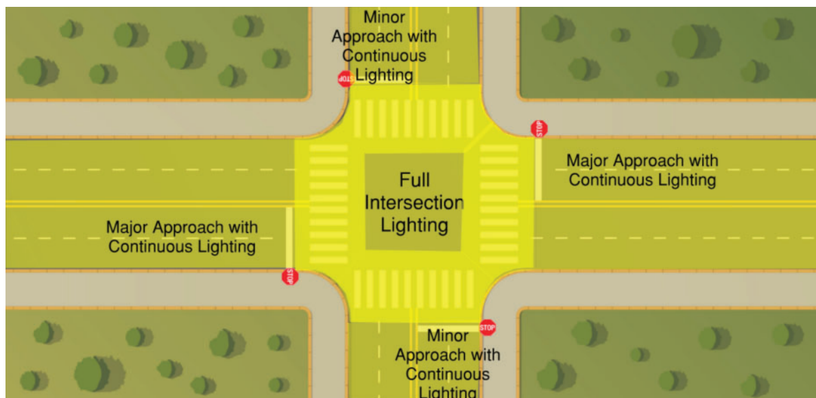
Figure 8-1. Illustration. Full Intersection Lighting with continuous lighting on both Major and Minor Approach Roadways.
