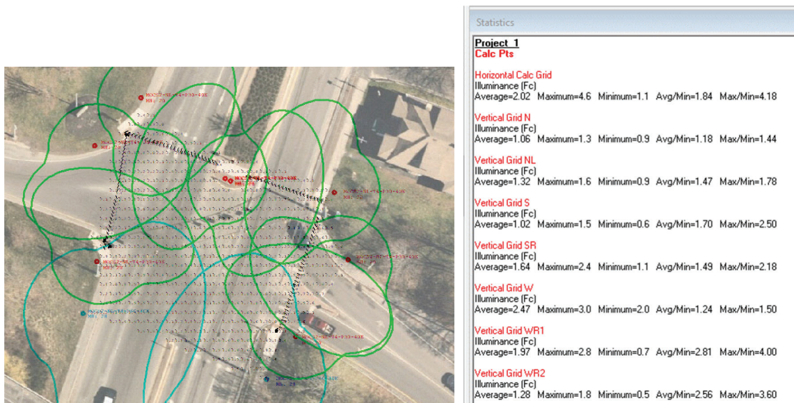
Figure 10-6. Illustration. The intersection of Main Street and Veterans Memorial Bridge in Lewiston, Maine.
