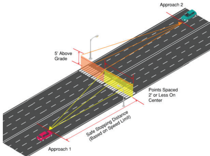
Figure 12-4. Illustration. One vertical illuminance calculation grid across only the approach lanes for wider roadways.
