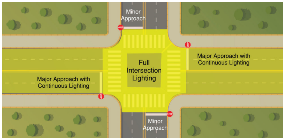
Figure 8-2. Illustration. Full Intersection Lighting with continuous lighting on the Major Approach Roadway.
