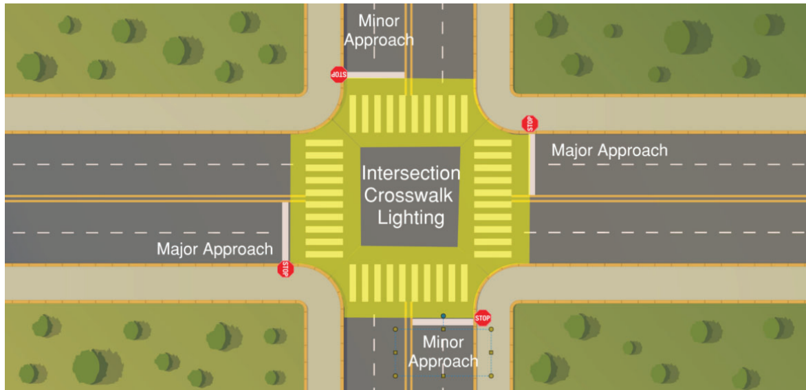
Figure 8-4. Illustration. Intersection Crosswalk Lighting.
