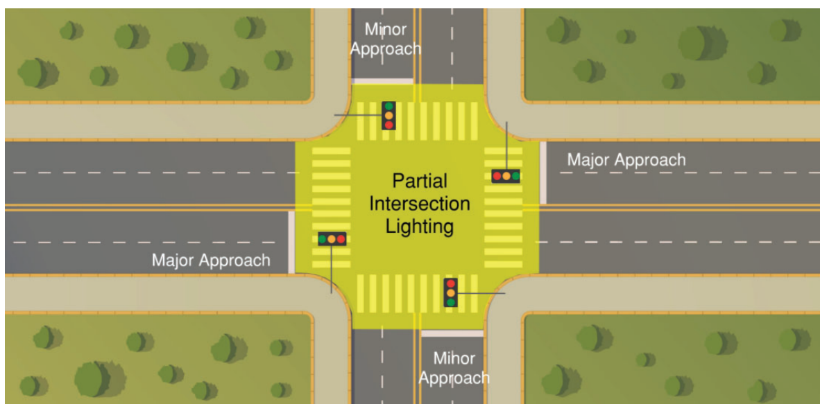
Figure 8-3. Illustration. Partial Intersection Lighting.
