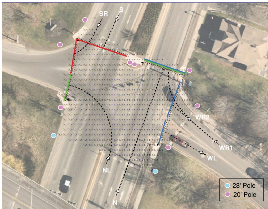
Figure 10-5. Illustration. Vertical calculation grids for Main Street (N, NL, S, SR) and the exit ramp from Veterans Memorial Bridge (WL, WR1, WR2). This is a unique intersection requiring a total of 7 vertical calculation grids based on the location of the crosswalks, one-way and two-way roadways, island, medians, dedicated left turn lanes, and dedicated right turn lanes.
