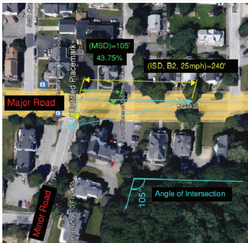
Figure 6-8. Illustration. AASHTO ISD Case B2 (Right Turn from Stop). Major Road (Main Street) and Minor Road (Frye Street) in Lewiston, Maine.
