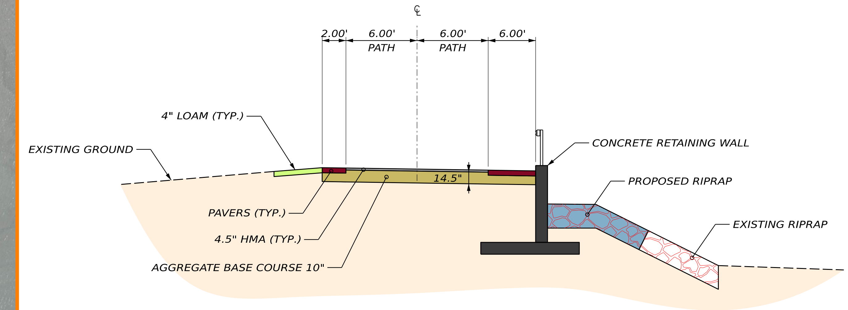
TYPICAL SECTION D-D PATH - RETAINING WALL
