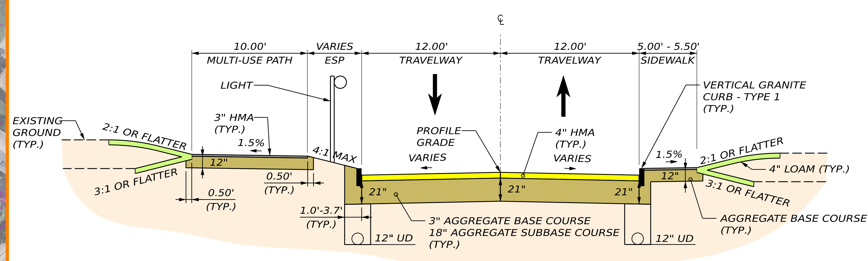
TYPICAL SECTION B-B SHERWOOD ST - 2 LANES
