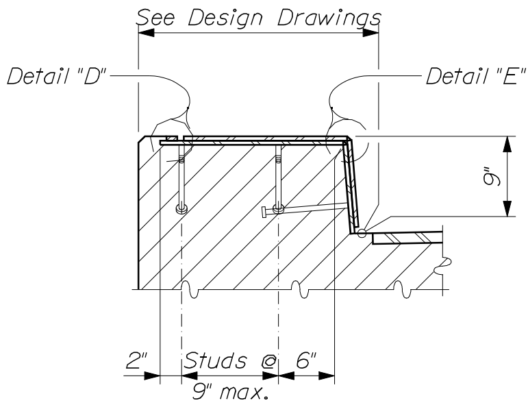
~ SECTION C-C ~
