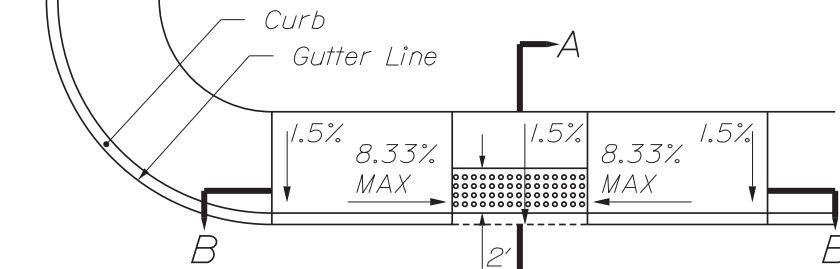
~ PLAN VIEW ~ (not to scale)
