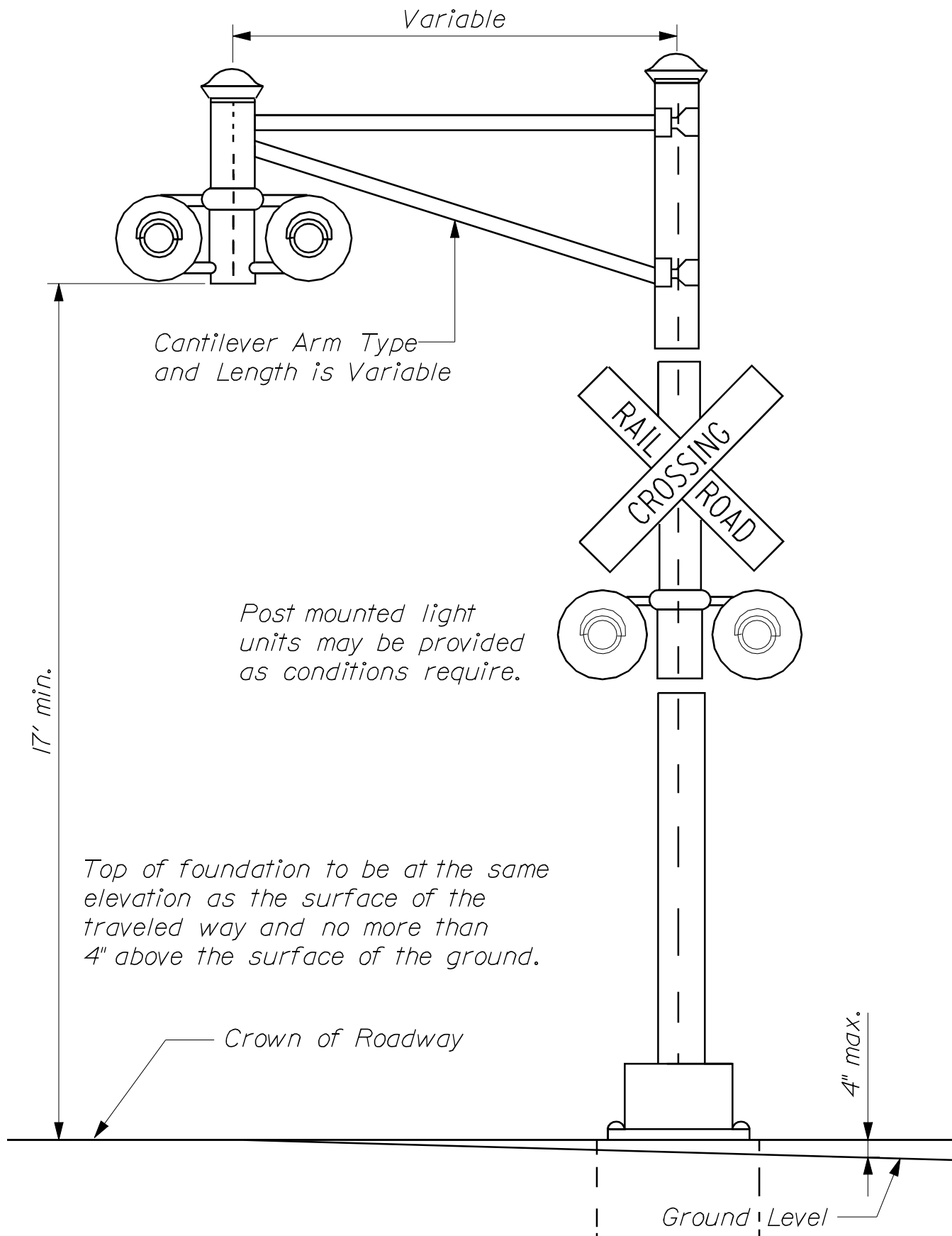
TYPICAL FLASHING LIGHT SIGNAL - CANTILEVER SUPPORTED
