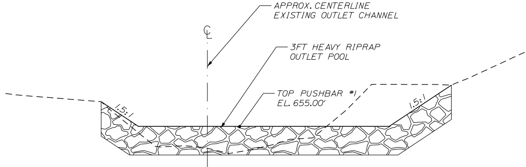
TYPICAL SECTION TOP PUSHBAR #1
