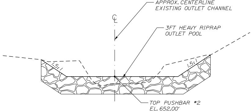
TYPICAL SECTION TOP PUSHBAR #2
