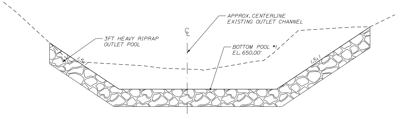
TYPICAL SECTION OUTLET POOL #1
