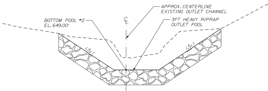
TYPICAL SECTION OUTLET POOL #2
