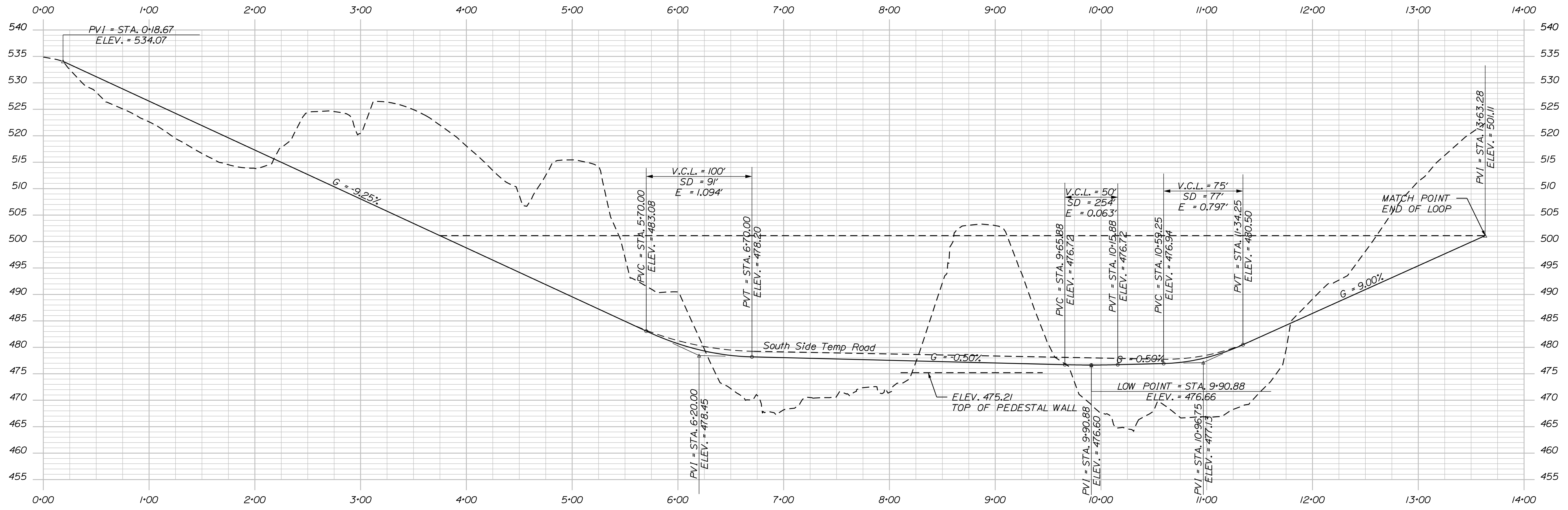
TEMPORARY ACCESS ROAD PROFILE
