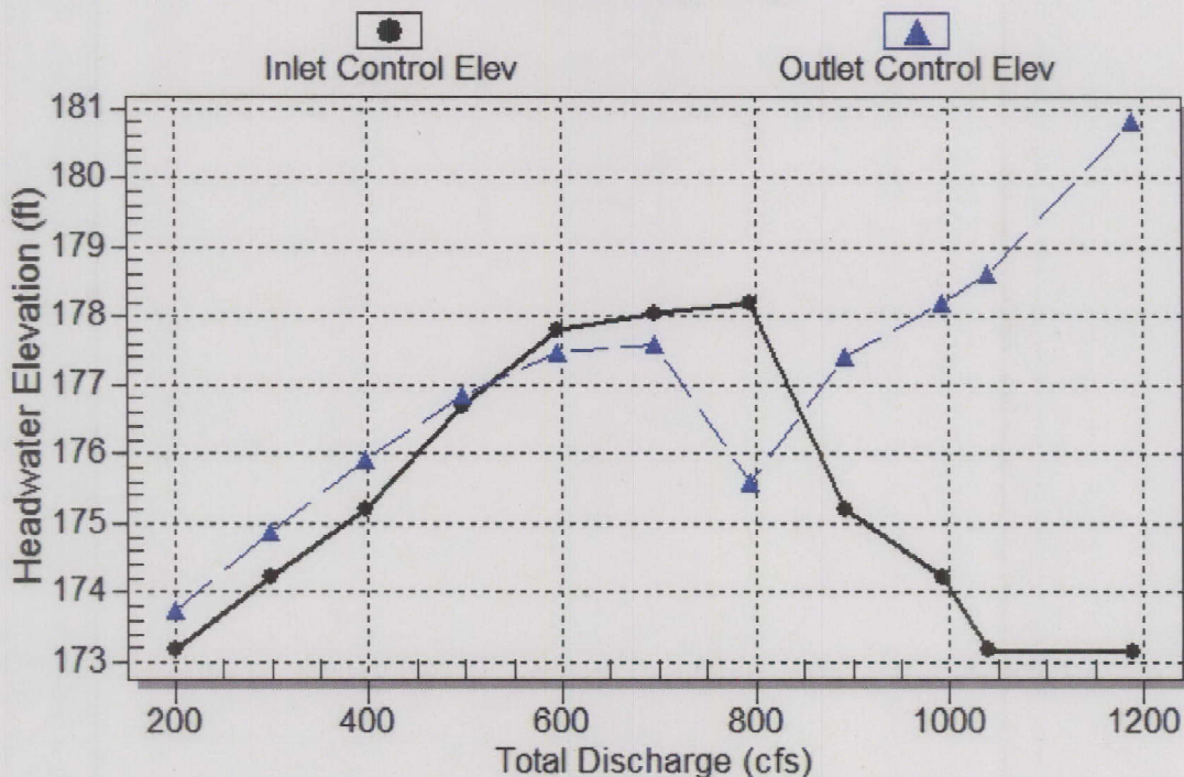
Culvert Performance Curve Plot: Existing Bridge Performance Curve Culvert: Existing Bridge
