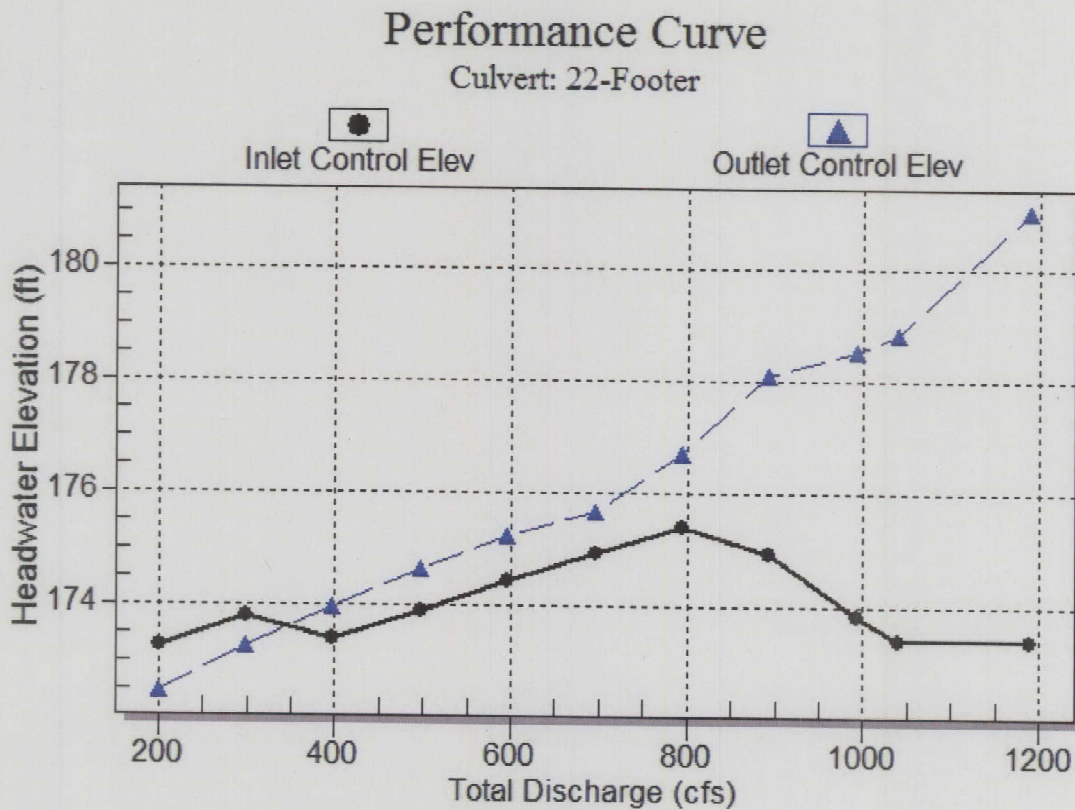
Culvert Performance Curve Plot: 22-Footer
