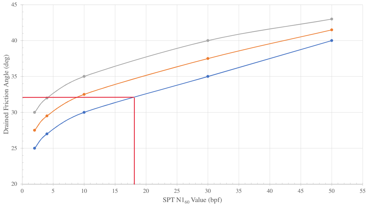
N160- \phi f Correlation (AASHTO Table 10.4.6.2.4-1)
