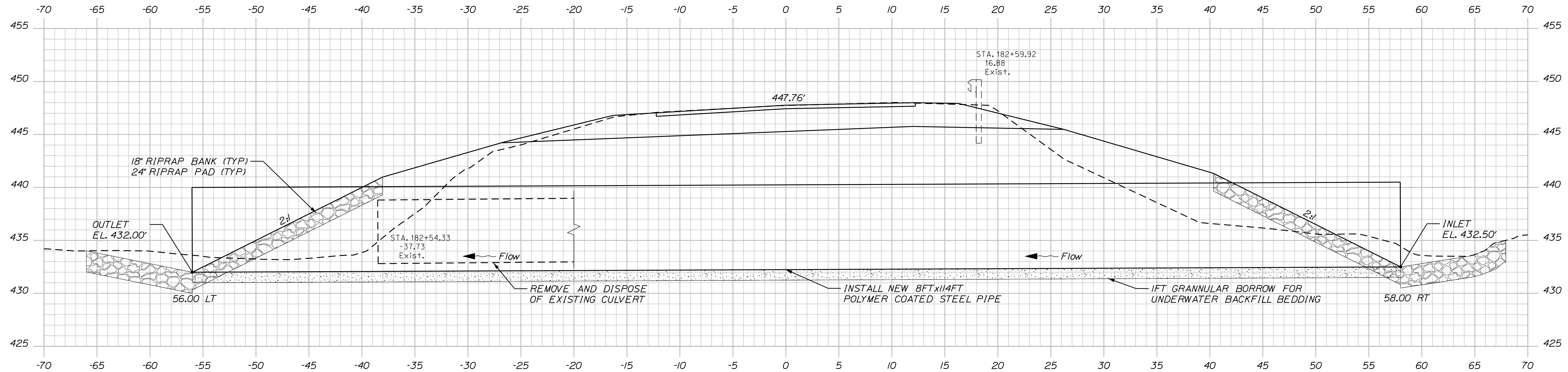
182+56.66 - CENTERLINE PIPE (SKEWED BACK LEFT 11°0'0.00")
