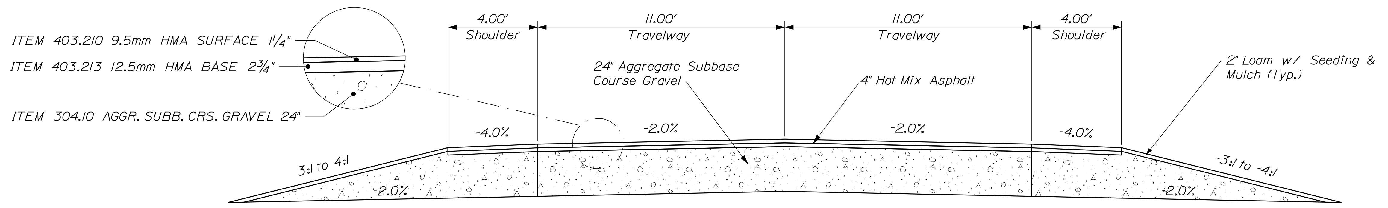
TYPICAL APPROACH DESIGN SECTION
