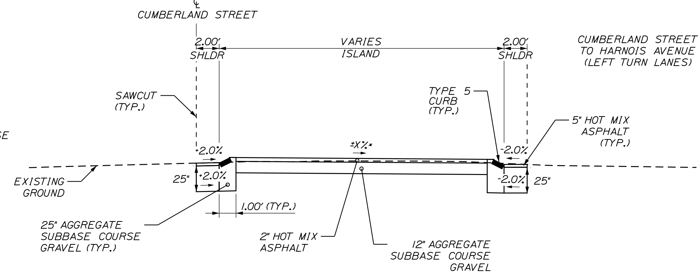
CUMBERLAND STREET & CUMBERLAND STREET TO HARNOIS AVENUE DETAIL F-F (N.T.S.)
