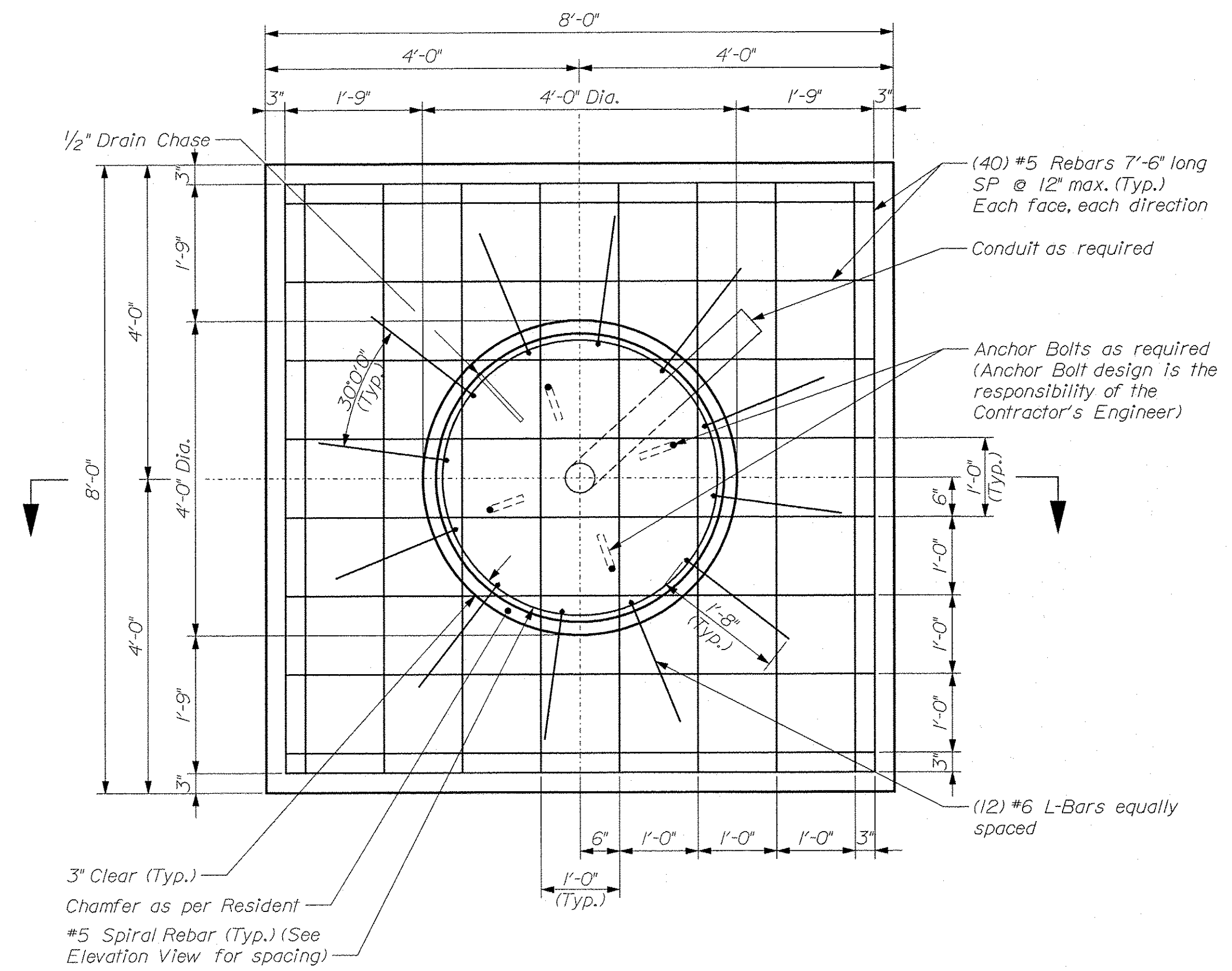
Spread Footing Plan View Scale: 3/4" = 1'-0"
