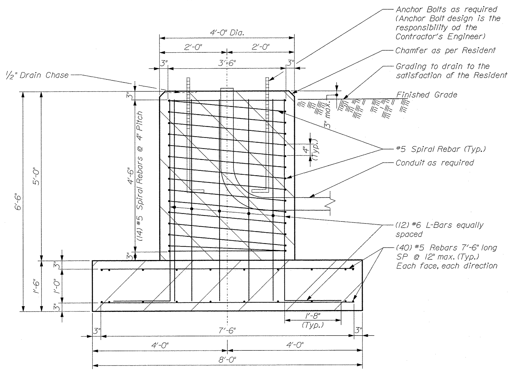
Spread Footing Elevation View Scale: 3/4" = 1'-0"
