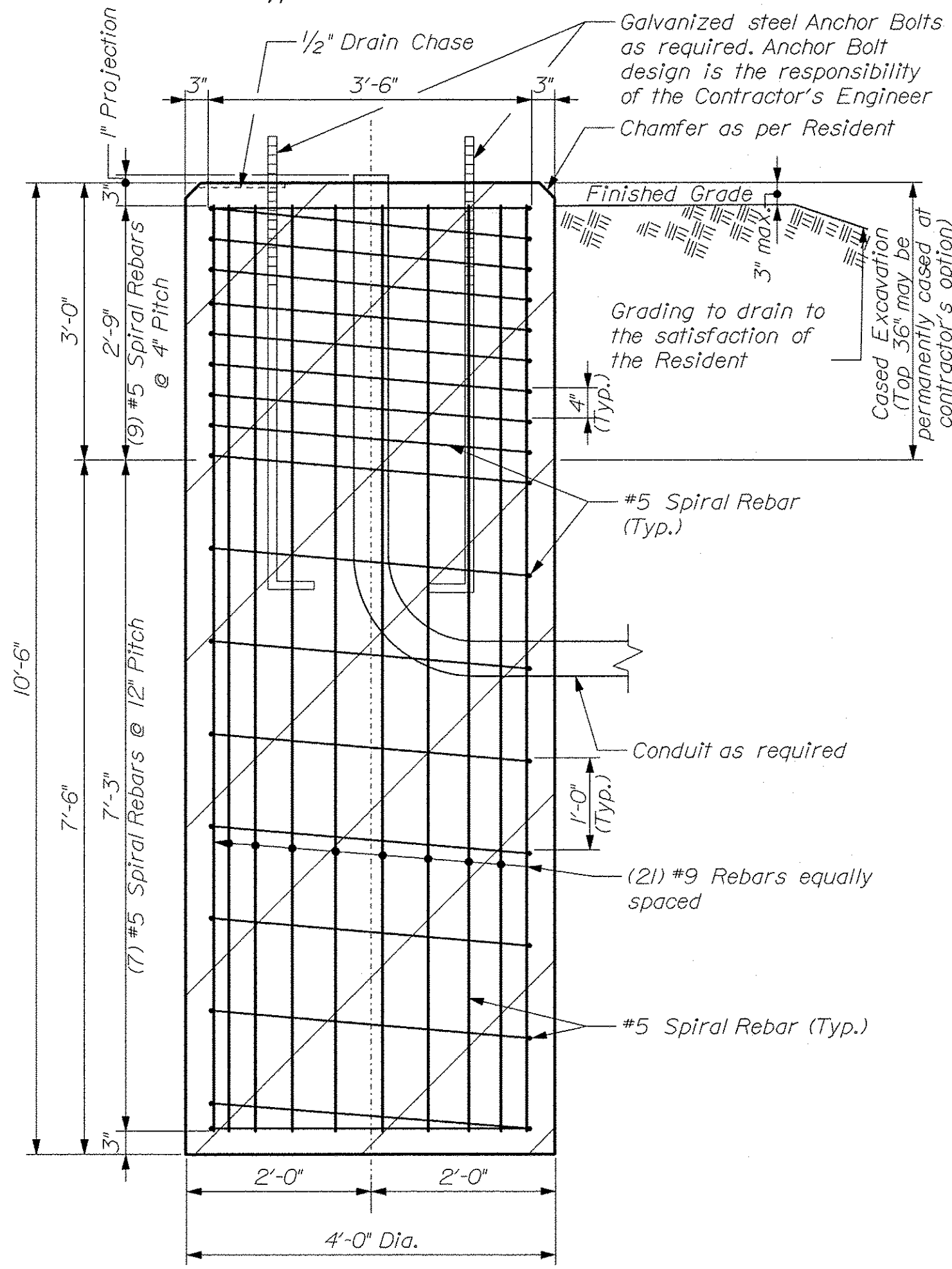
Drilled Shaft Elevation View Scale: 3/4" = 1'-0" MAST ARM B Sta. 42+39, 11.8' Lt.
