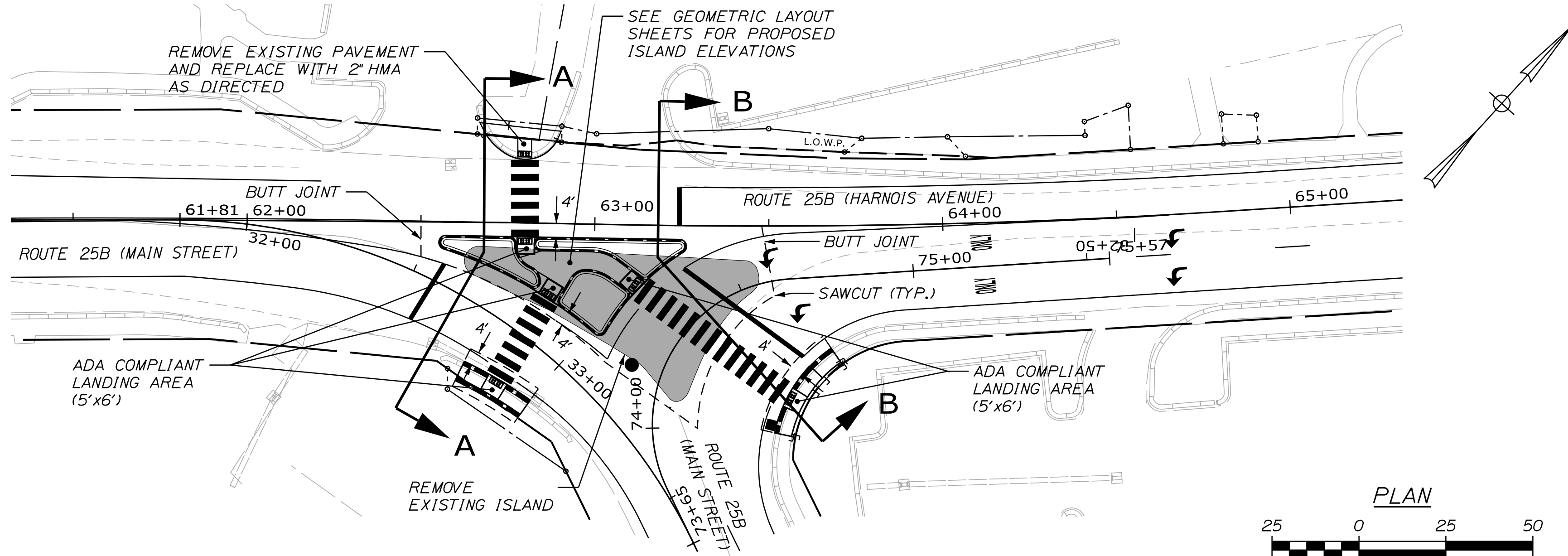
HARNOIS AVENUE & MAIN STREET PLAN
