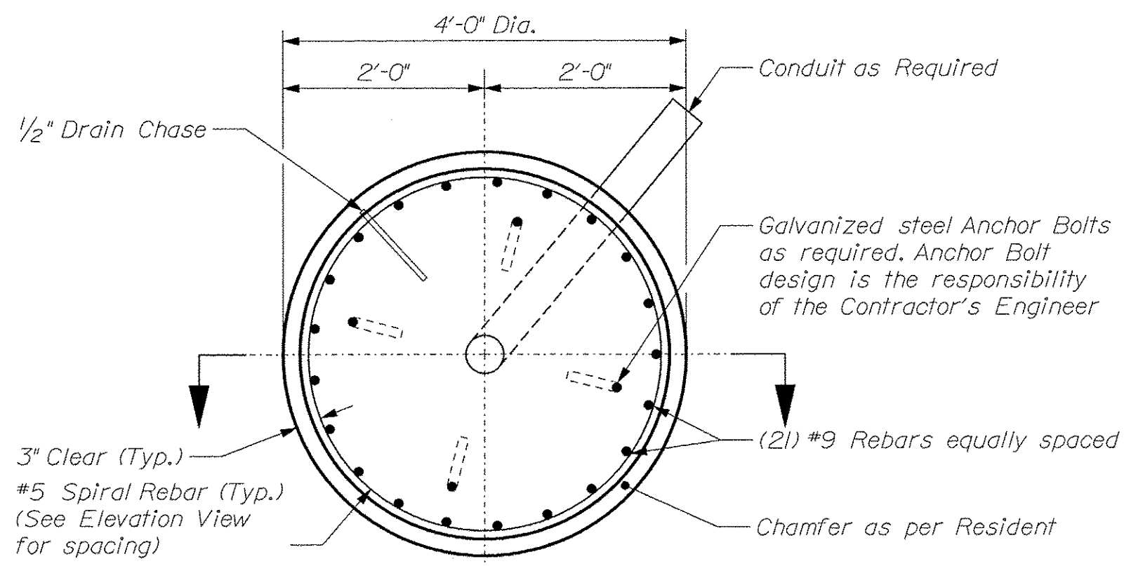
Drilled Shaft Plan View Scale: 3/4" = 1'-0"
