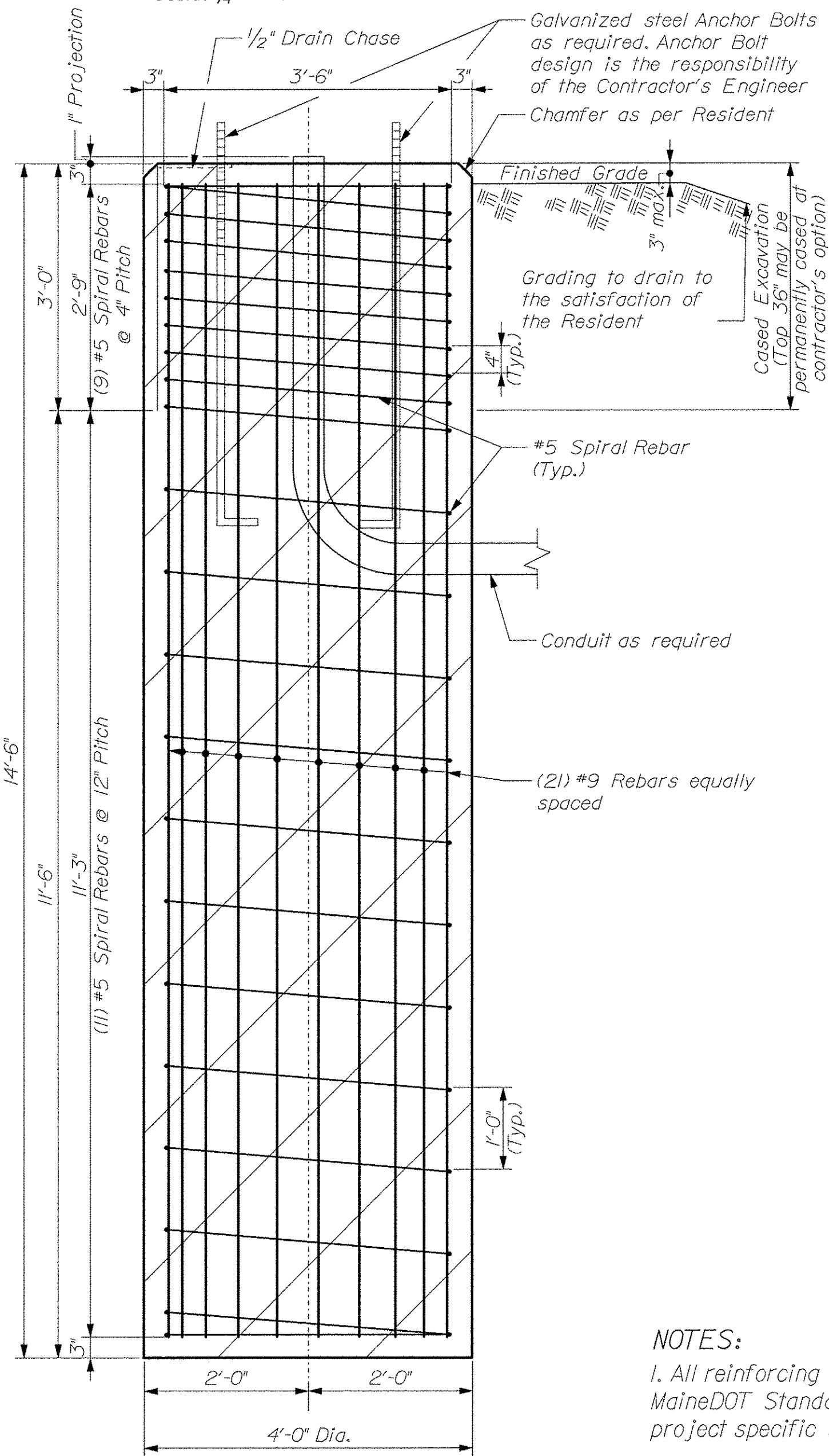
Drilled Shaft Elevation View Scale: 3/4" = 1'-0" MAST ARM A Sta. 21+82, 20.8' Rt.
