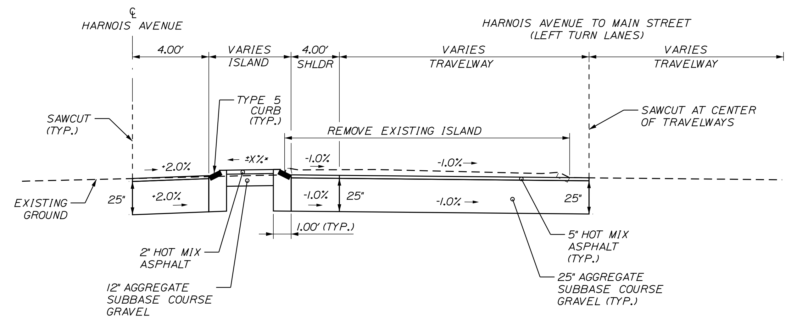
HARNOIS AVENUE & HARNOIS AVENUE TO MAIN STREET DETAIL B-B (N.T.S.)
