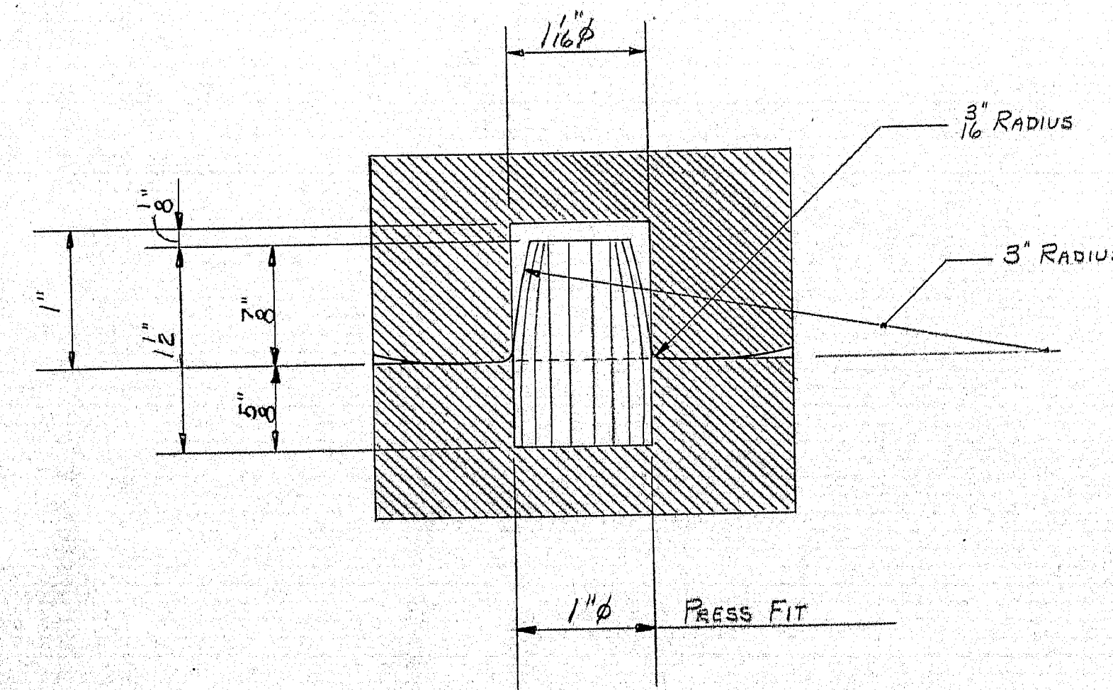
DOWEL DETAIL
