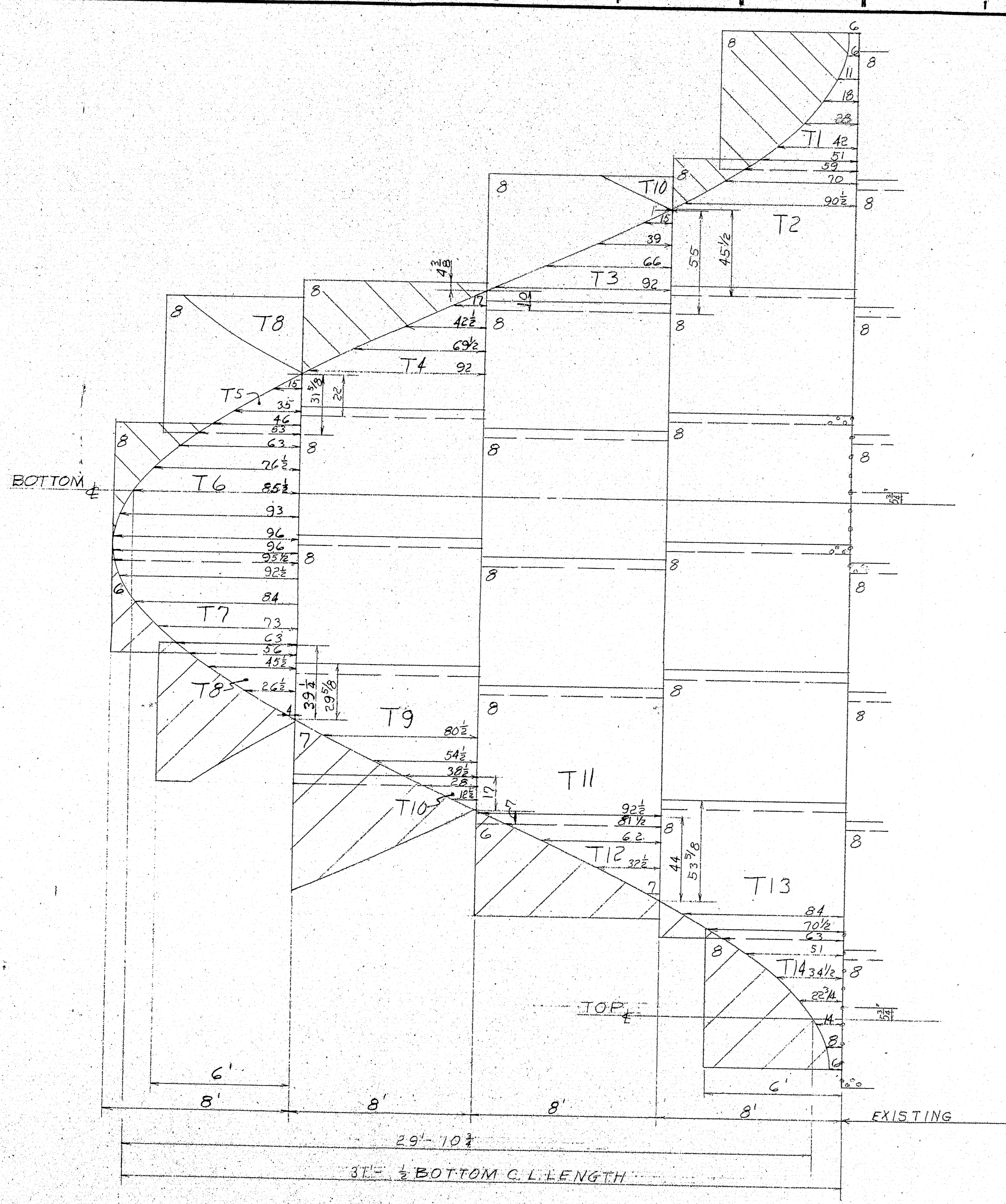
CUTTING DIAGRAM & PLATE LAYOUT-INSIDE VIEW
