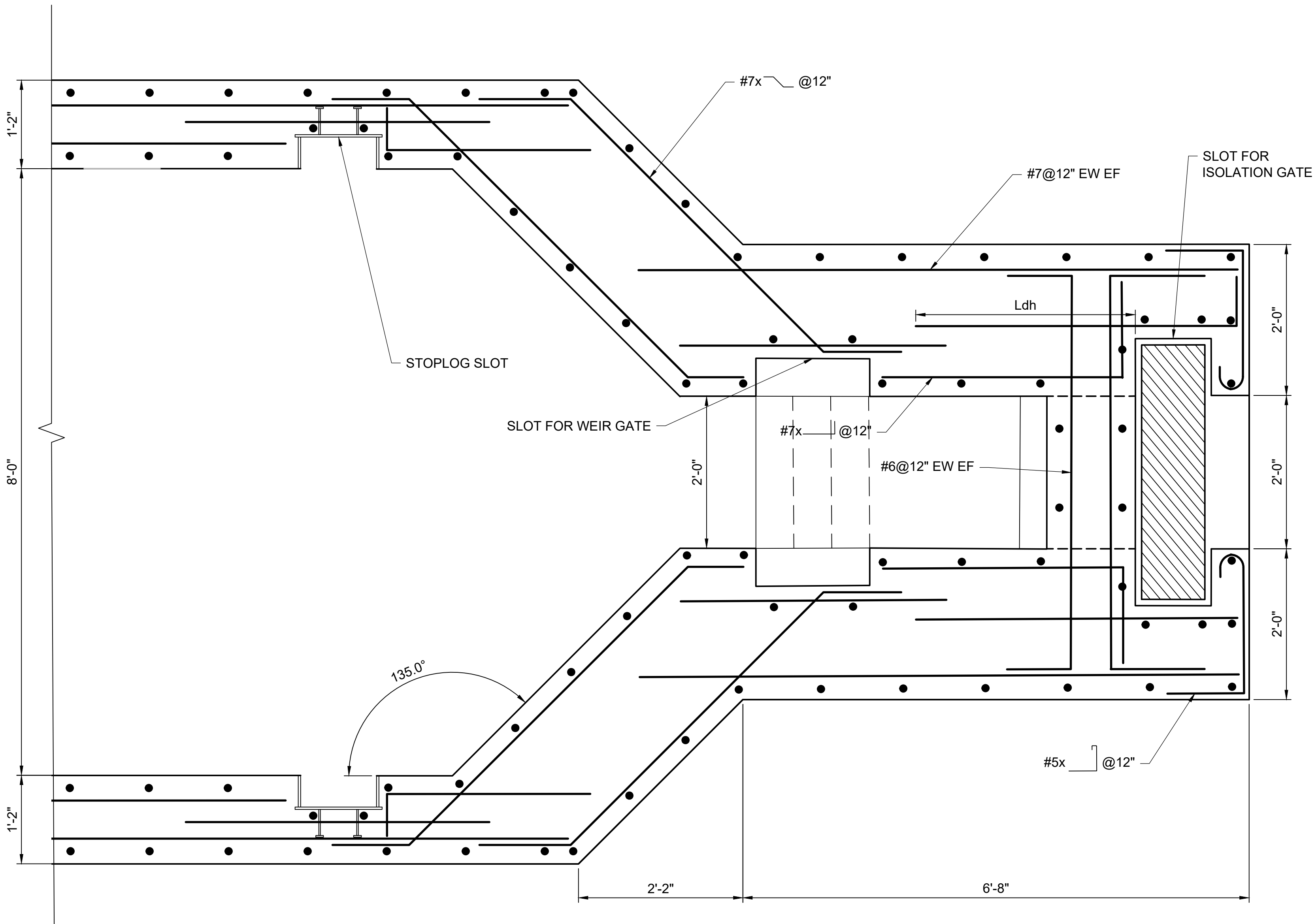
1 S-143 ENLARGED PLAN SCALE: 1"=1'-0" 0 1' 2'
