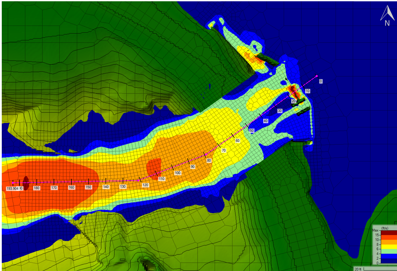
Figure B - 2. Overview of flow speeds at Chase Mills Bridge for the 100-year return period peak flow for proposed conditions; alignment station is based on the longitudinal profile in the hydraulic report Figure 9.
