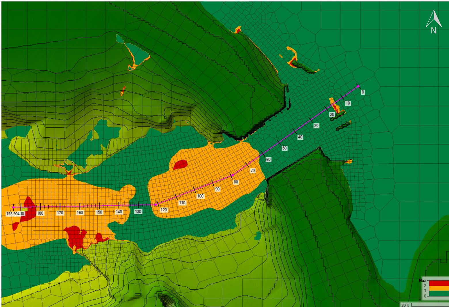
Figure B - 5. Overview of Froude number at Chase Mills Bridge for the 100-year return period peak flow for existing conditions; alignment station is based on the longitudinal profile in the hydraulic report Figure 9.
