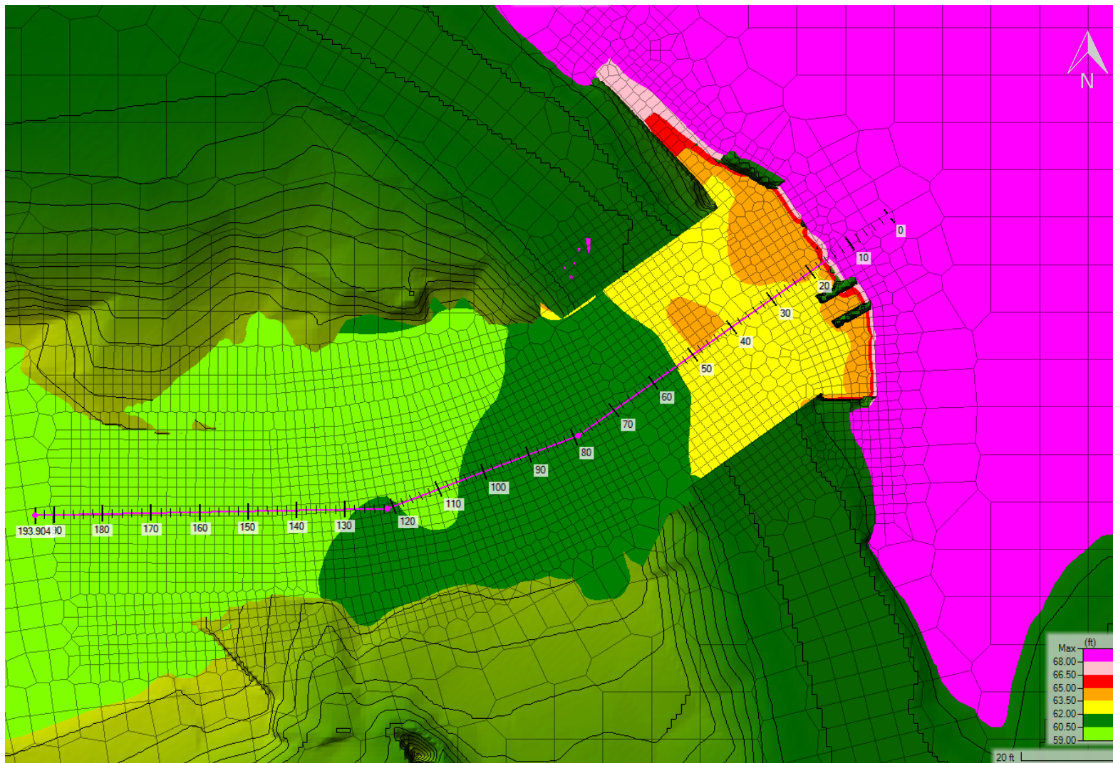
Figure B - 4. Overview of WSELs at Chase Mills Bridge for the 100-year return period peak flow for proposed conditions; alignment station is based on the longitudinal profile in the hydraulic report Figure 9.
