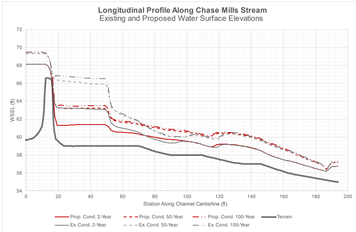
Figure 9. Simulated WSELs along the Chase Mills Stream alignment for the 2-, 50-, and 100-year return period peak flows for existing and proposed conditions
