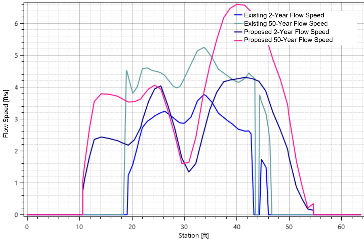
Figure 7. Simulated flow speeds at the upstream cross-section for the 2- and 50-year return period peak flows for existing and proposed conditions
