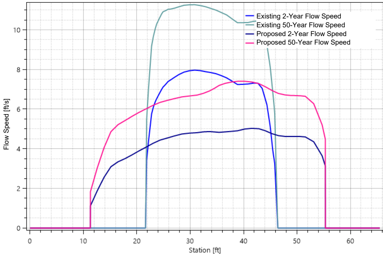
Figure 8. Simulated flow speeds at the downstream cross-section for the 2- and 50-year return period peak flows for existing and proposed conditions
