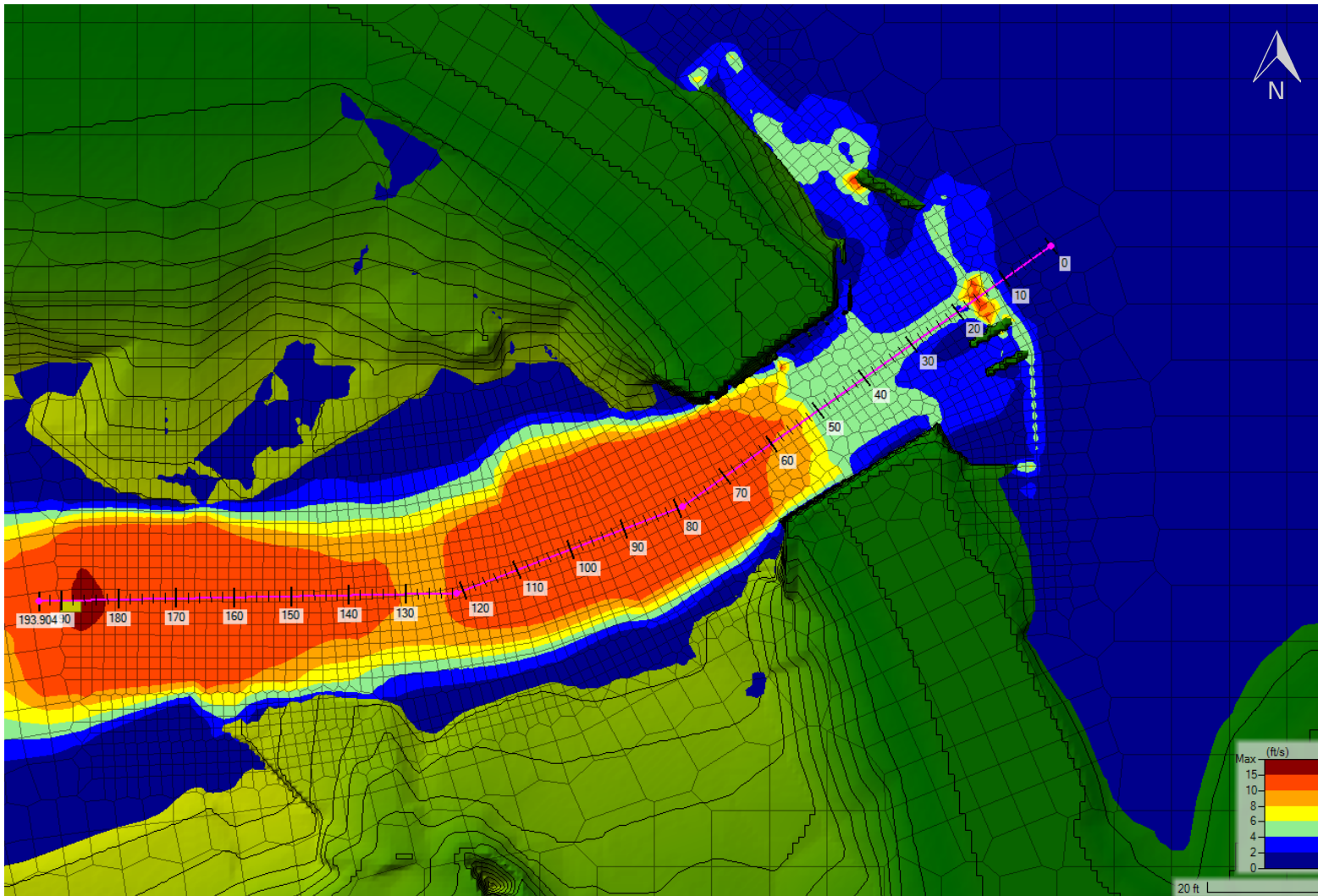
Figure B - 1. Overview of flow speeds at Chase Mills Bridge for the 100-year return period peak flow for existing conditions; alignment station is based on the longitudinal profile in the hydraulic report Figure 9.
