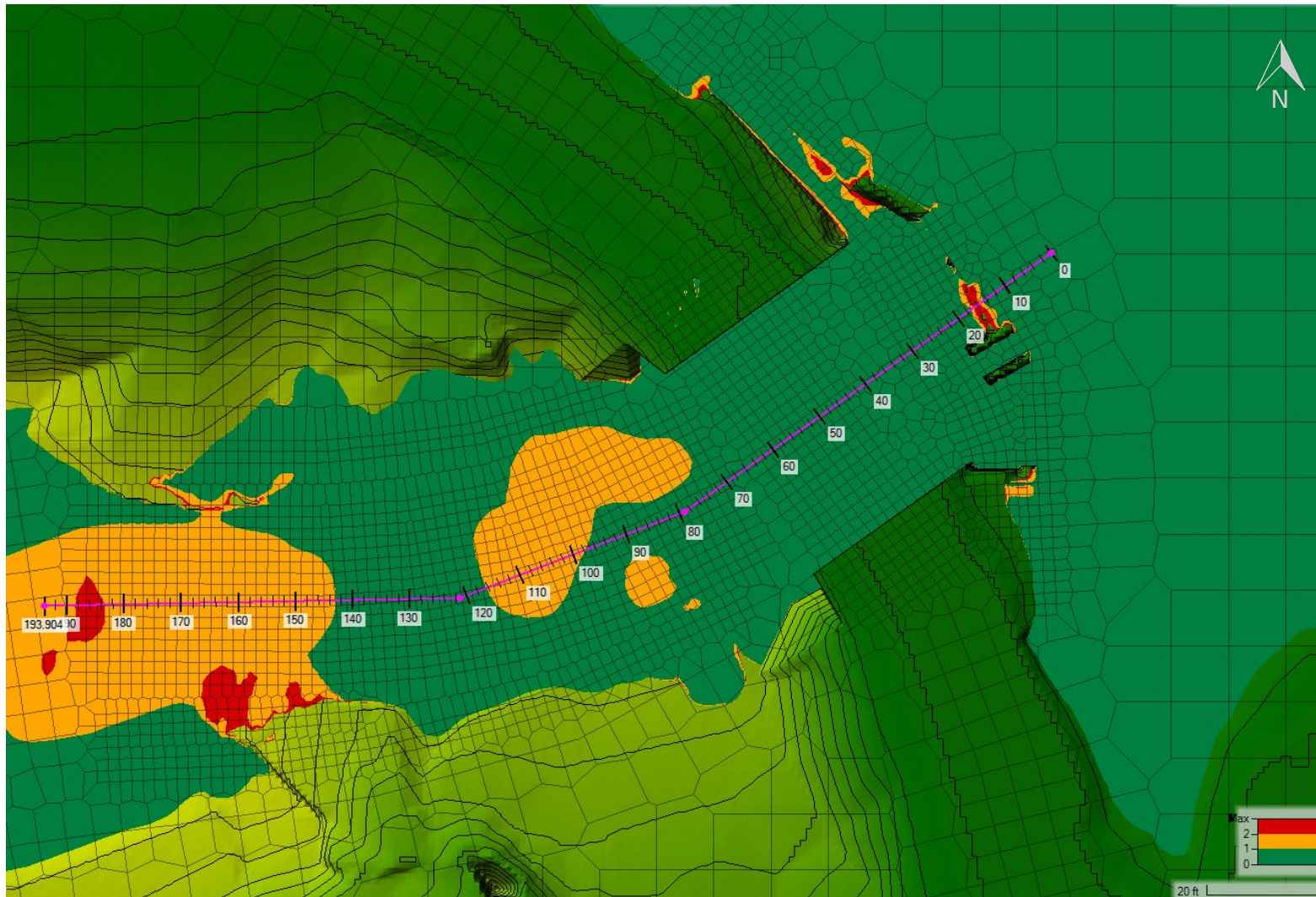
Figure B - 6. Overview of Froude number at Chase Mills Bridge for the 100-year return period peak flow for proposed conditions; alignment station is based on the longitudinal profile in the hydraulic report Figure 9.
