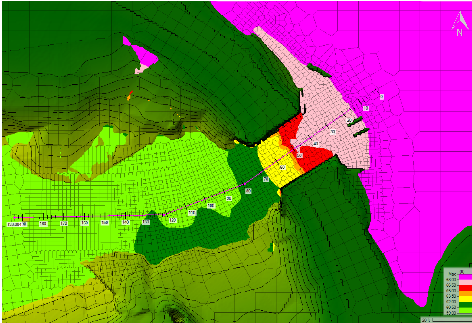
Figure B - 3. Overview of WSELs at Chase Mills Bridge for the 100-year return period peak flow for existing conditions; alignment station is based on the longitudinal profile in the hydraulic report Figure 9.
