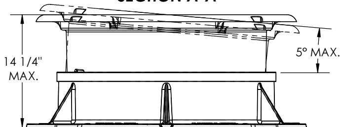
FRONT VIEW (SHOWING MAXIMUM TIP @ 5° ANGLE)
