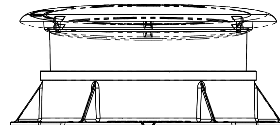
SIDE VIEW (SHOWING MAXIMUM TIP @ 5° ANGLE)
