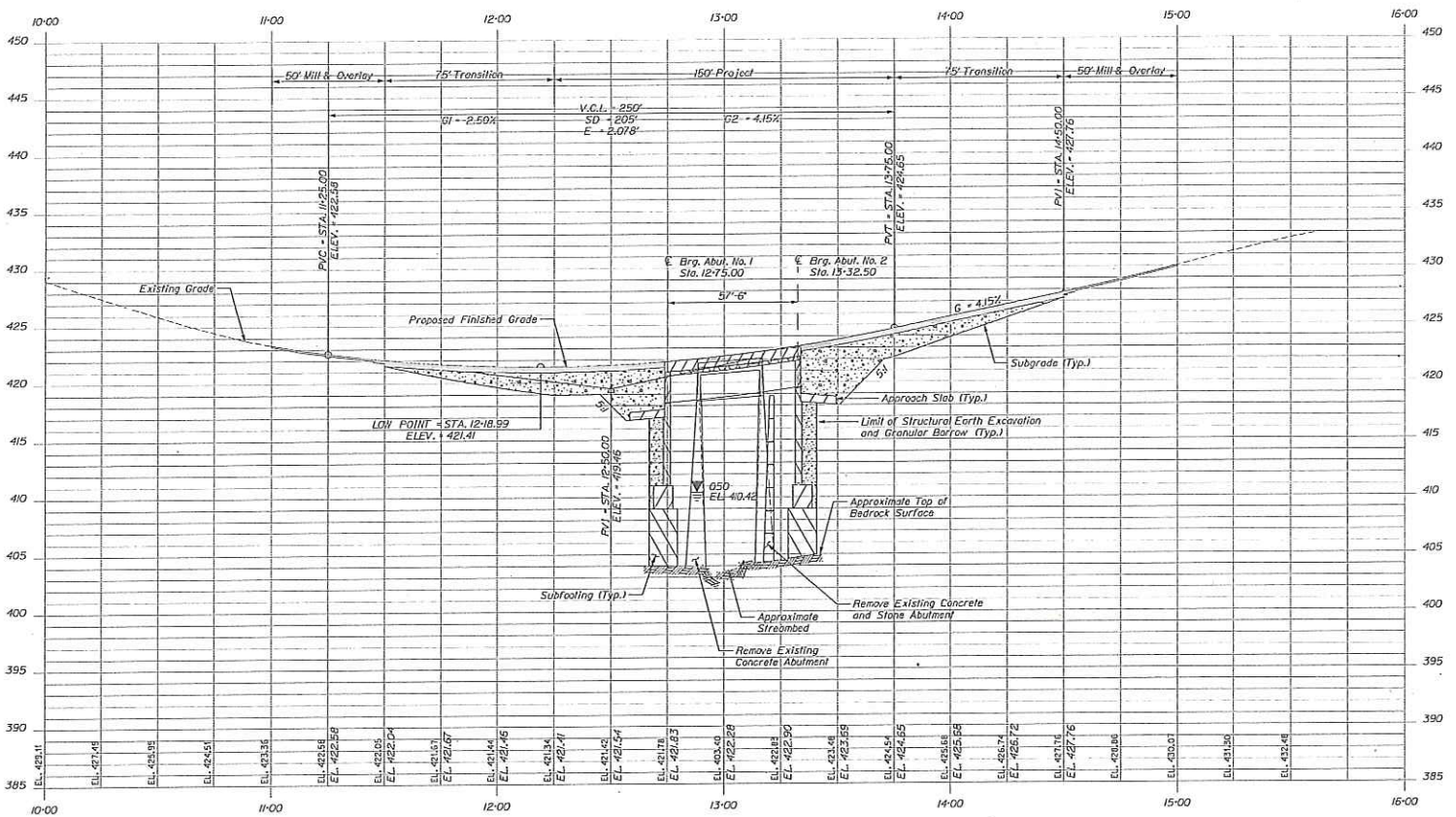
PROFILE
