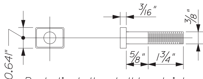
~ BOLT HOLE PUNCHING PLAN FOR EXTRUDED ALUMINUM PLANKS ~
