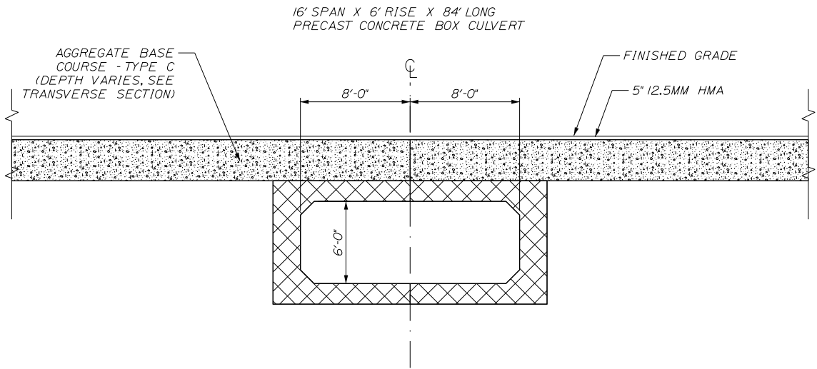
PRECAST CONCRETE BOX CULVERT TRANSVERSE SECTION (ALONG CULVERT CL) NOT TO SCALE
