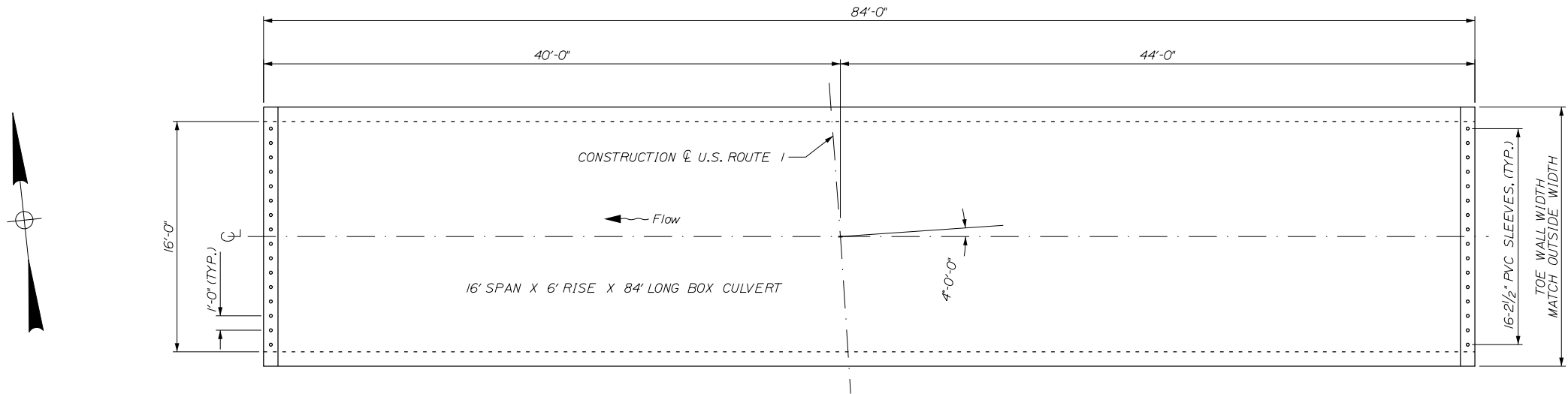
PRECAST CONCRETE BOX CULVERT PLAN VIEW NOT TO SCALE
