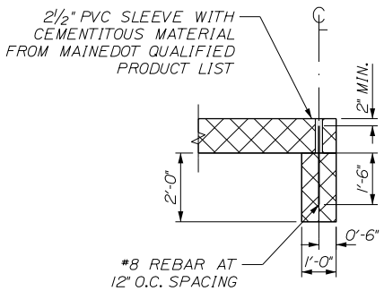
PRECAST CONCRETE TOE WALL DETAIL NOT TO SCALE
