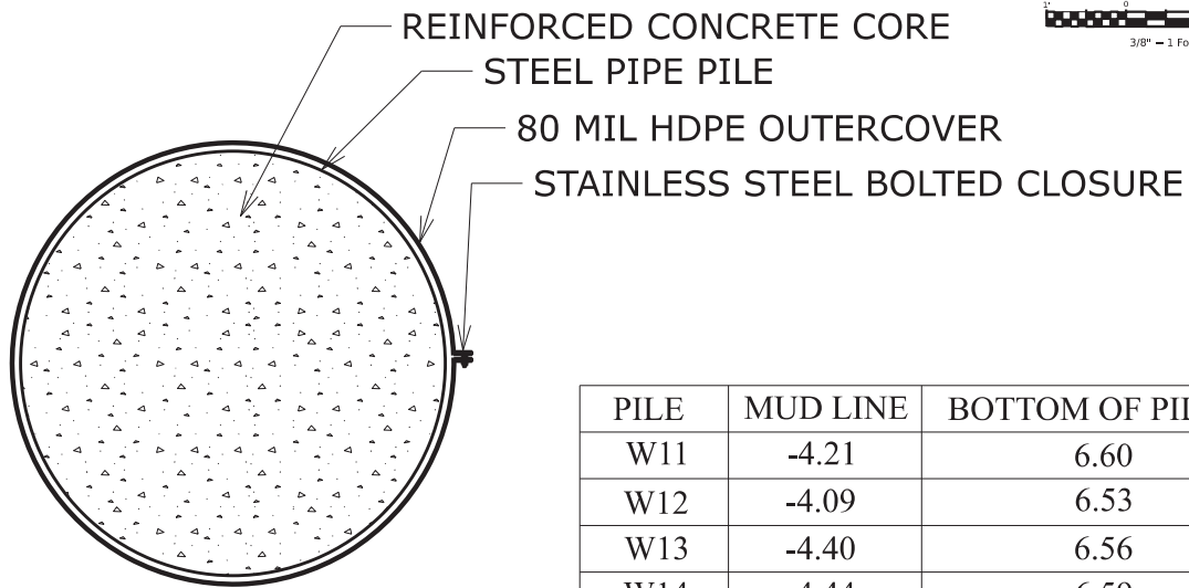
PILE SECTION
