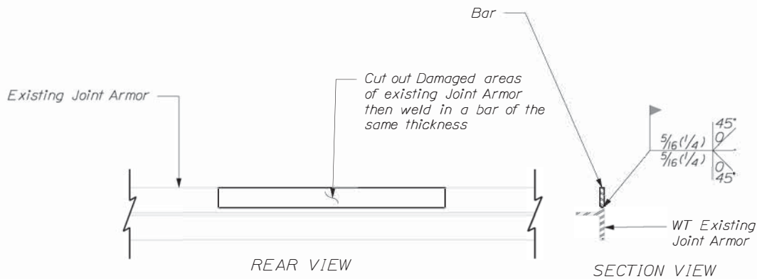
COMPRESSION SEAL JOINT ARMOR REPAIR
