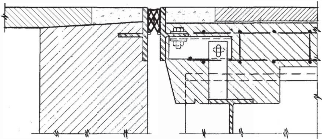
SECTION VIEW - EXISTING BRIDGE JOINTS
