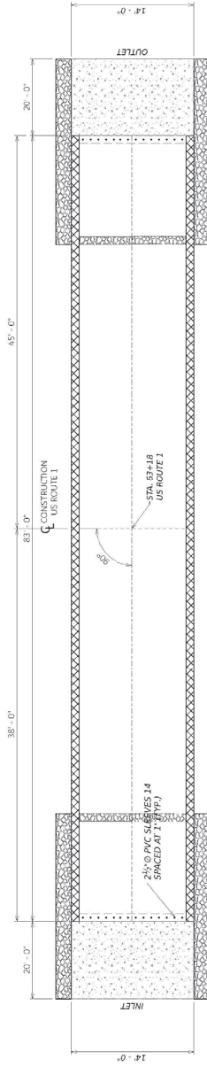
TYPICAL PRECAST CONCRETE BOX CULVERT PLAN VIEW
