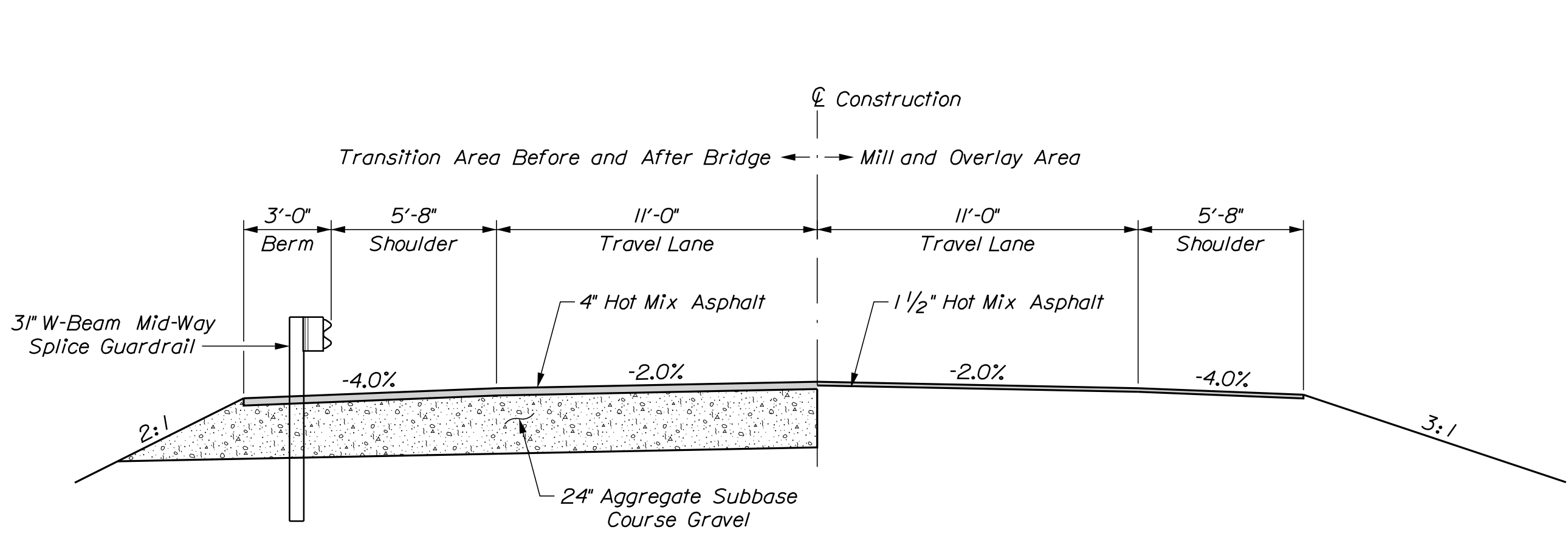
TYPICAL APPROACH HALF SECTIONS
