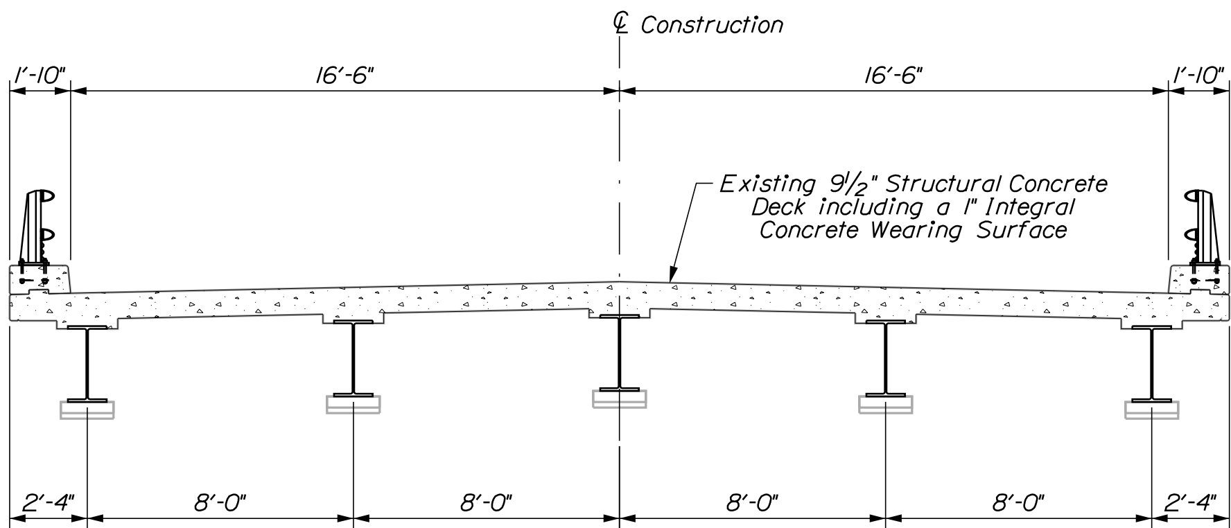
EXISTING BRIDGE SECTION
