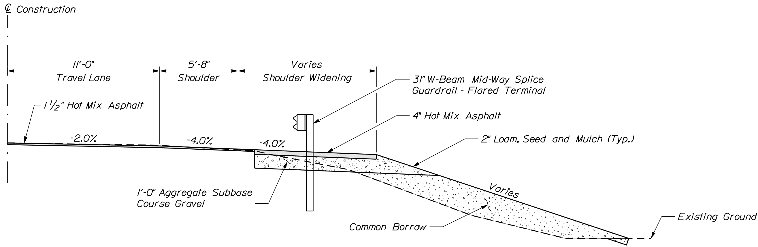
TYPICAL SHOULDER WIDENING SECTION
