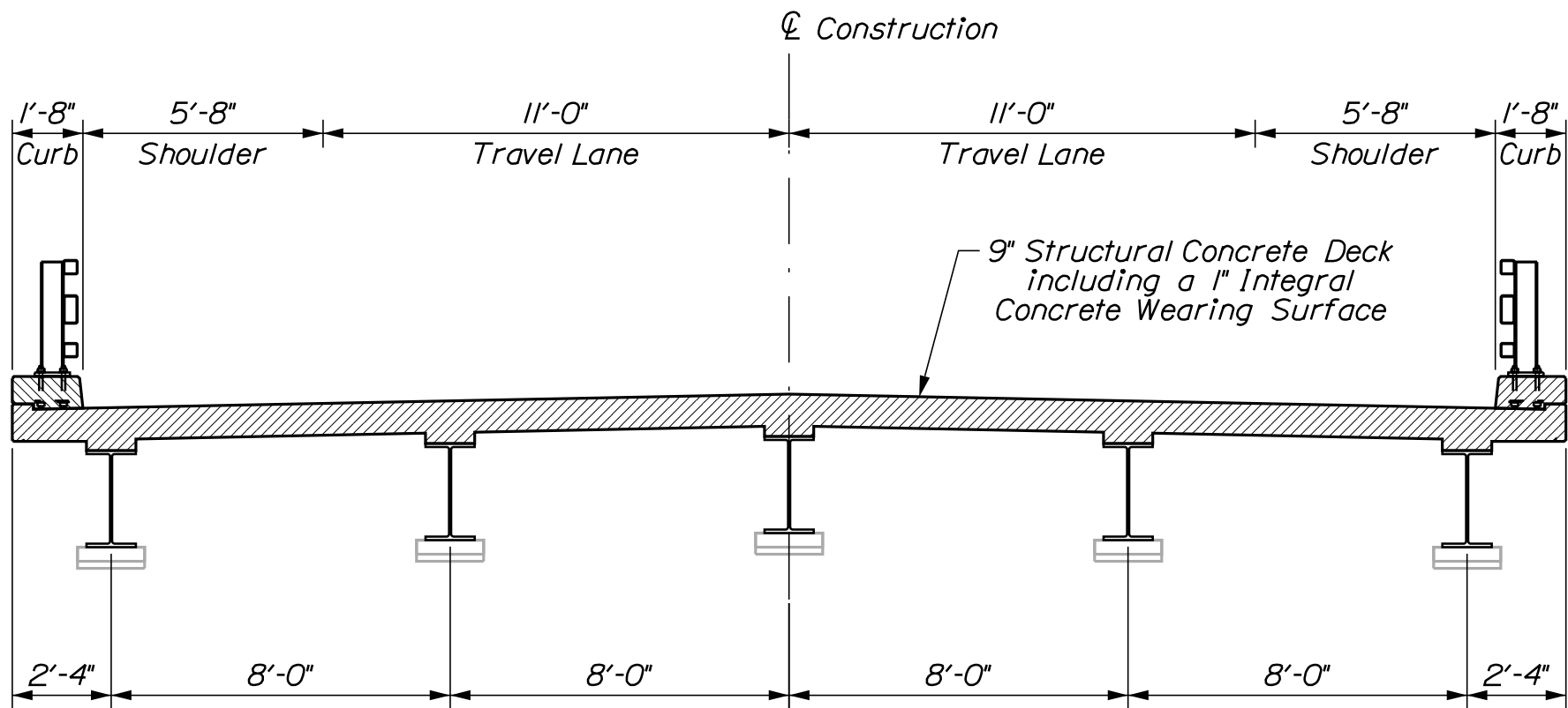
PROPOSED BRIDGE SECTION
