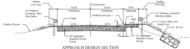
APPROACH DESIGN SECTION
