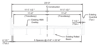
SECTION - EXISTING STRUCTURE
