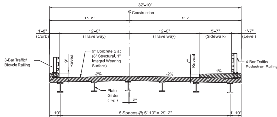
SECTION - PROPOSED STRUCTURE
