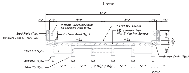
EXISTING BRIDGE TYPICAL
