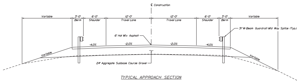
TYPICAL APPROACH SECTION
