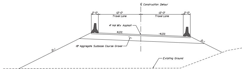
TEMPORARY DETOUR SECTION
