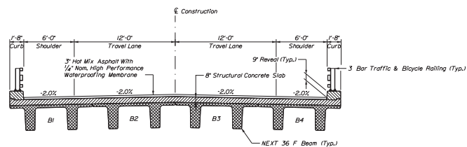
TRANSVERSE SECTION NEXT 36 F BEAM
