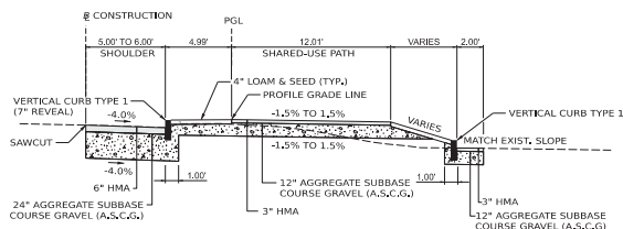
SHARED USE PATH STA. 101+50.00 TO STA. 102+50.00 STA. 112+00.00 TO STA. 116+25.00
