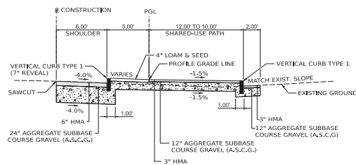
SHARED USE PATH STA. 122+25.00 TO STA. 124+25.00
