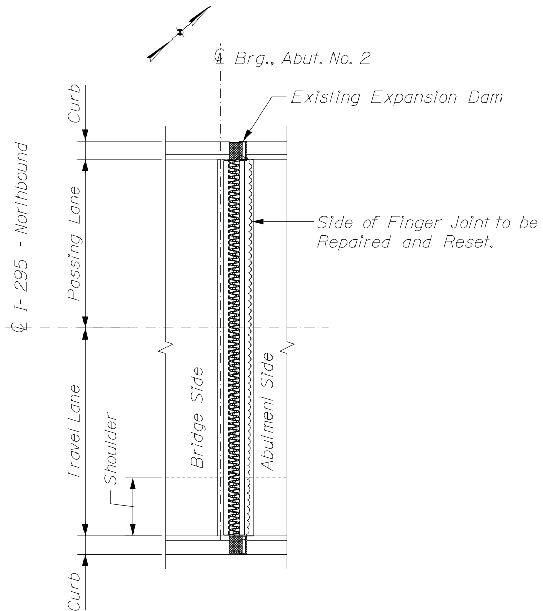
PLAN VIEW OF JOINT REPAIR
