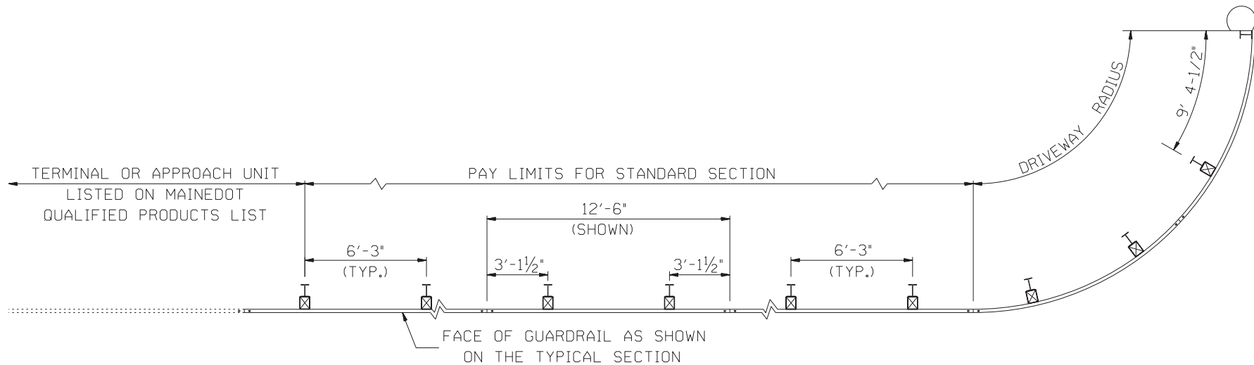
PLAN
