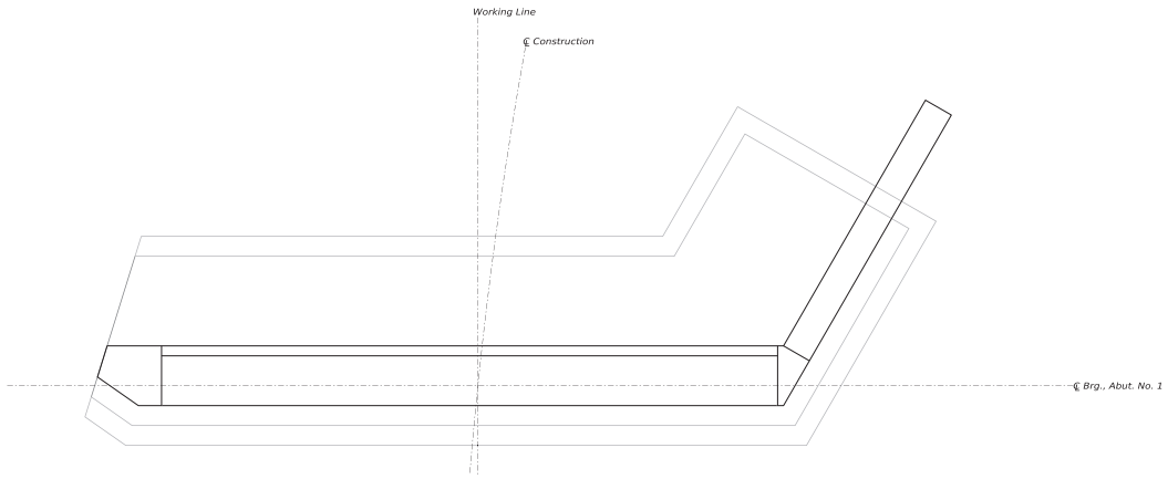
ABUTMENT NO. 1 REINFORCING PLAN
