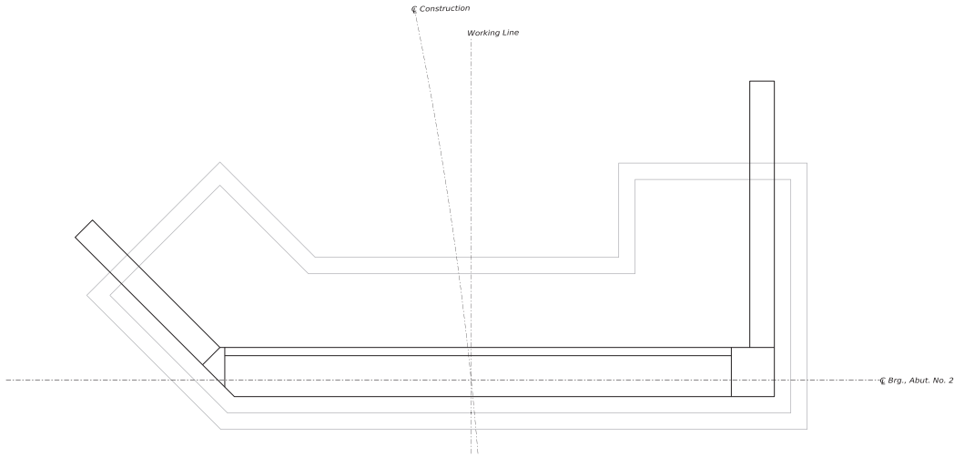
ABUTMENT NO. 2 REINFORCING PLAN
