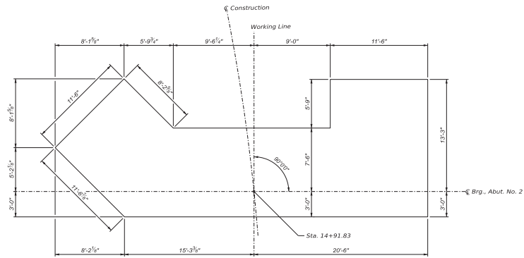
ABUTMENT NO. 2 SEAL PLAN
