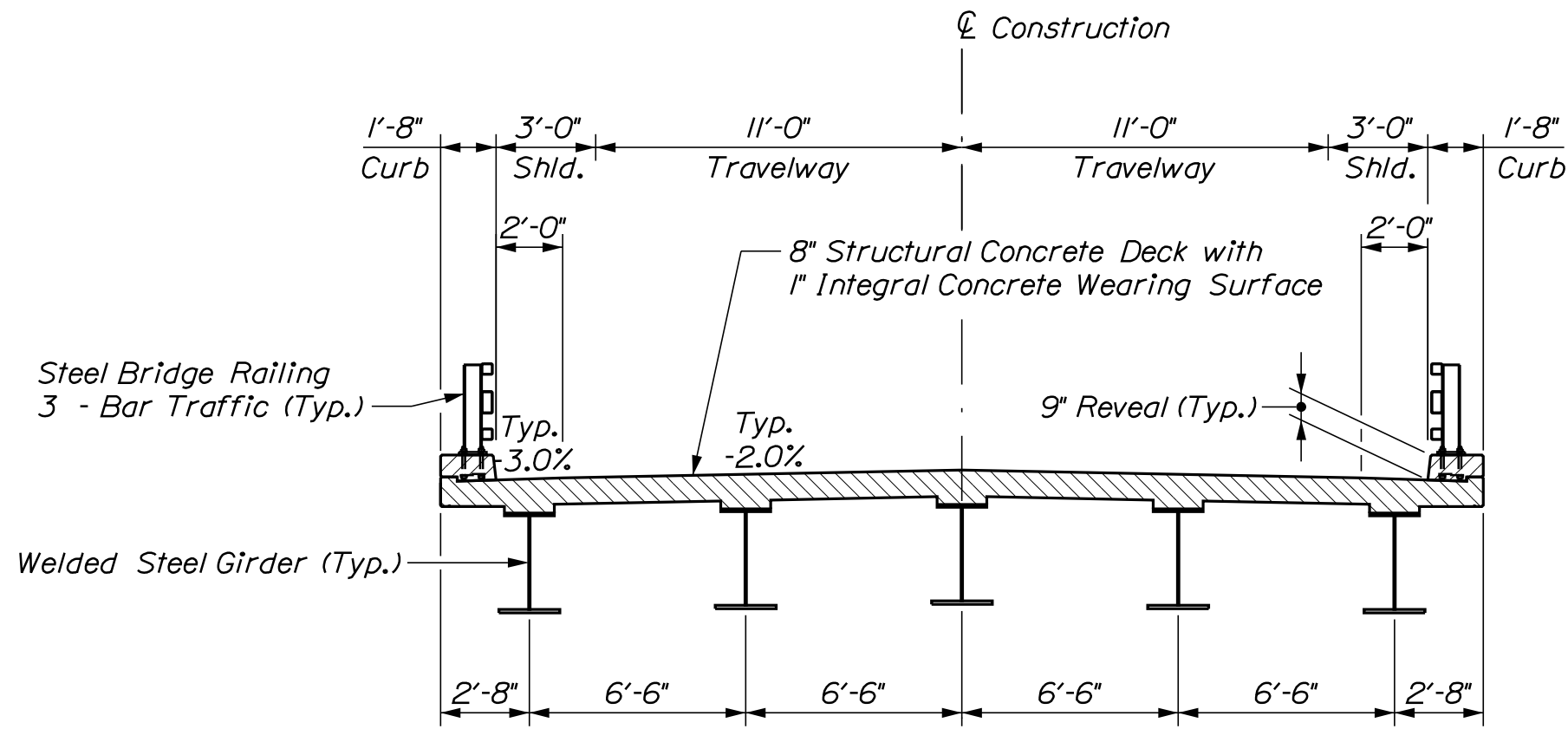
PROPOSED TYPICAL BRIDGE SECTION (Final deck section after milling procedure)
