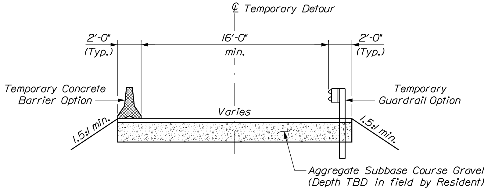
TEMPORARY DETOUR APPROACH SECTION
