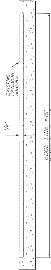
SECTION C-C (NOT TO SCALE)
