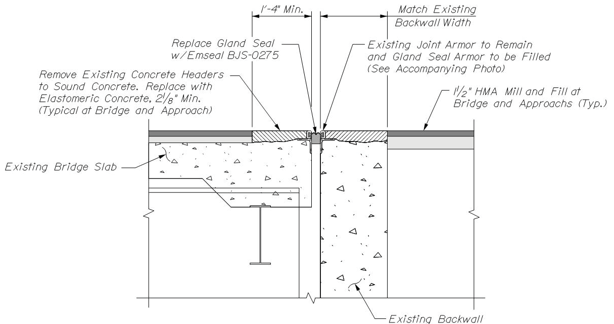
BRIDGE JOINT MODIFICATION (Type 3)
