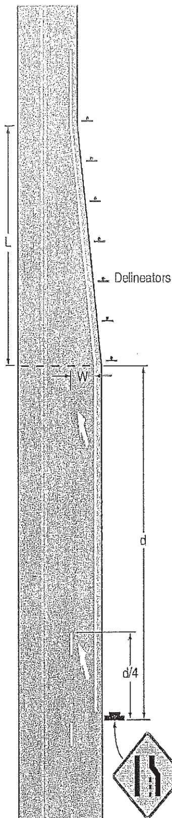
A – Lane reduction
