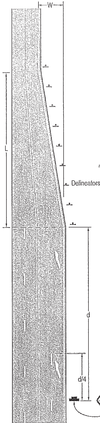
B – Lane reduction with lateral shift to the left
