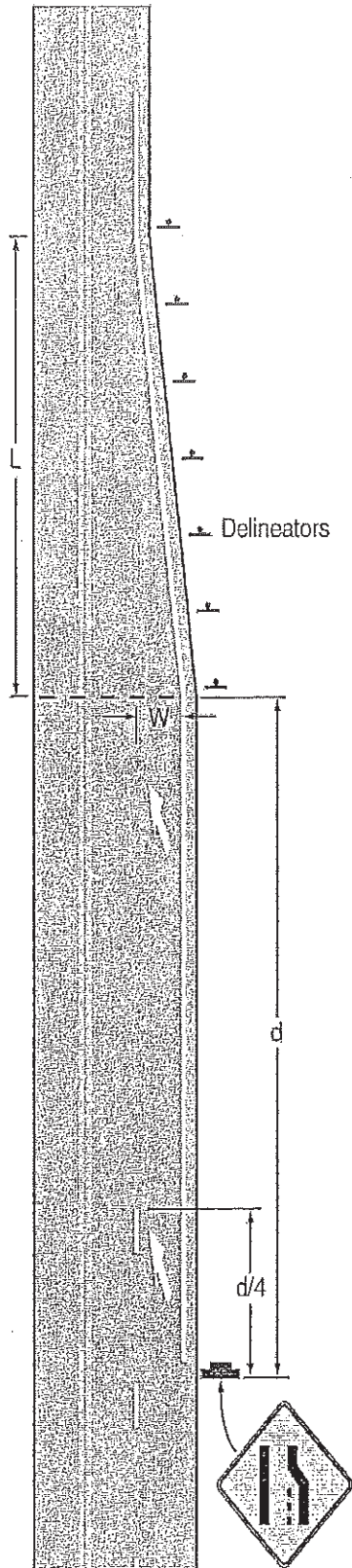
A – Lane reduction
