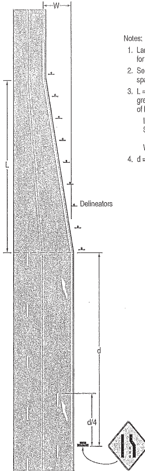
B – Lane reduction with lateral shift to the left
