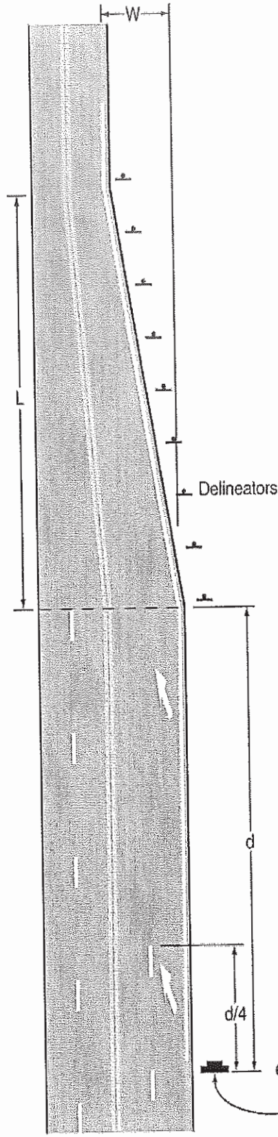
B – Lane reduction with lateral shift to the left
