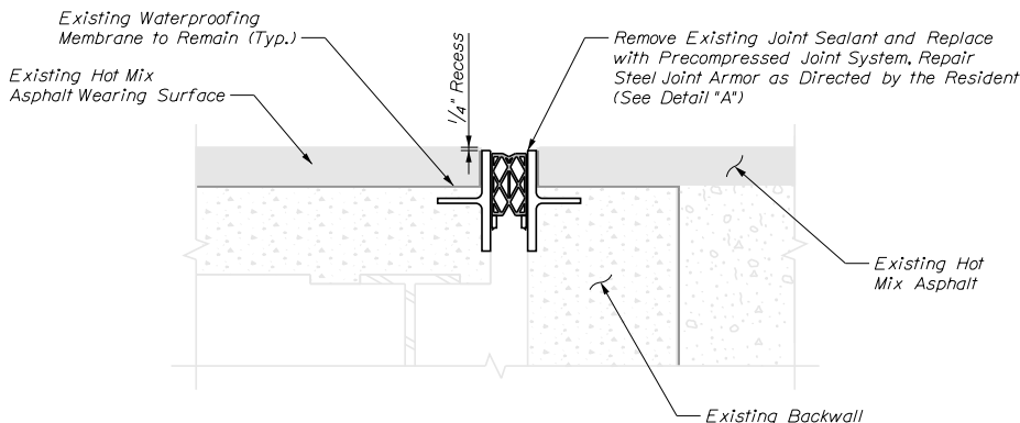
BRIDGE JOINT MODIFICATION TYPE 2
