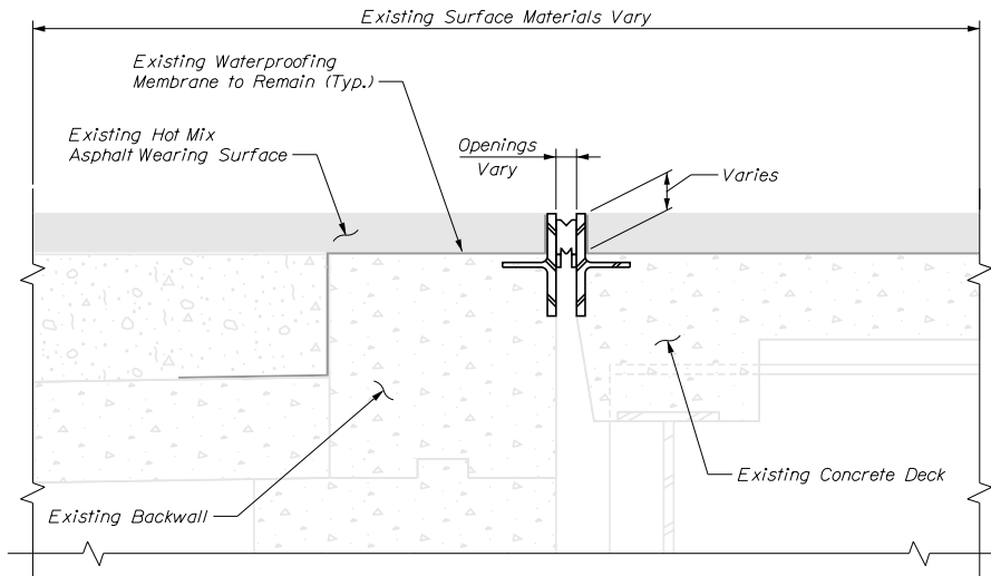
EXISTING COMPRESSION SEAL JOINT
