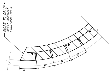
CONNECTION DETAIL
