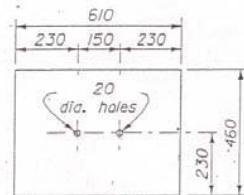
Steel plate 6 thickness
