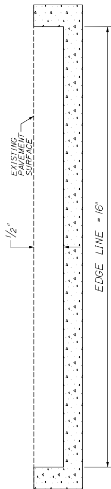
SECTION B-B (NOT TO SCALE)
