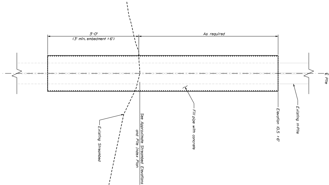
PILE JACKET DETAIL (Typical on piles)
