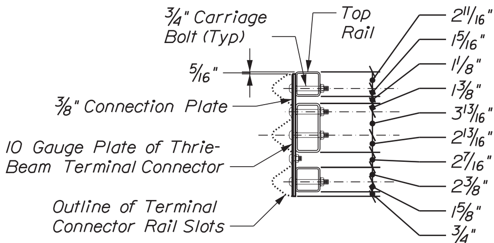
~ SECTION B-B (CONNECTION PLATE) ~
